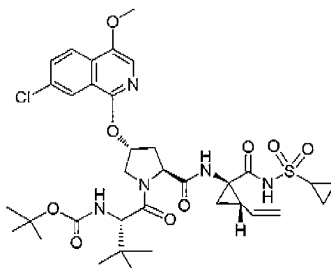
BMS-650032 (Asunaprevir)
