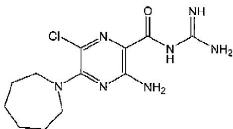
BIT-225
