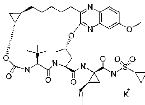
MK-5172
