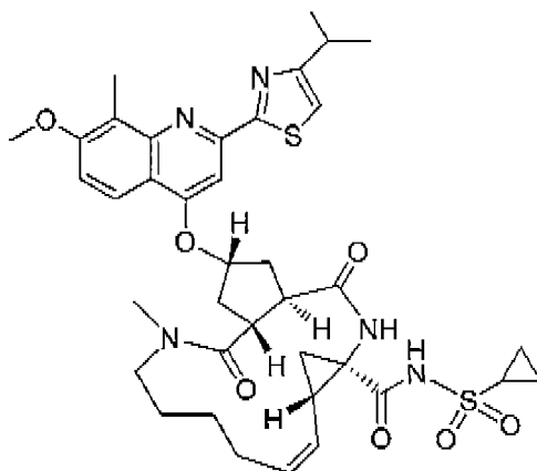
TMC-435 (TMC-435350)
