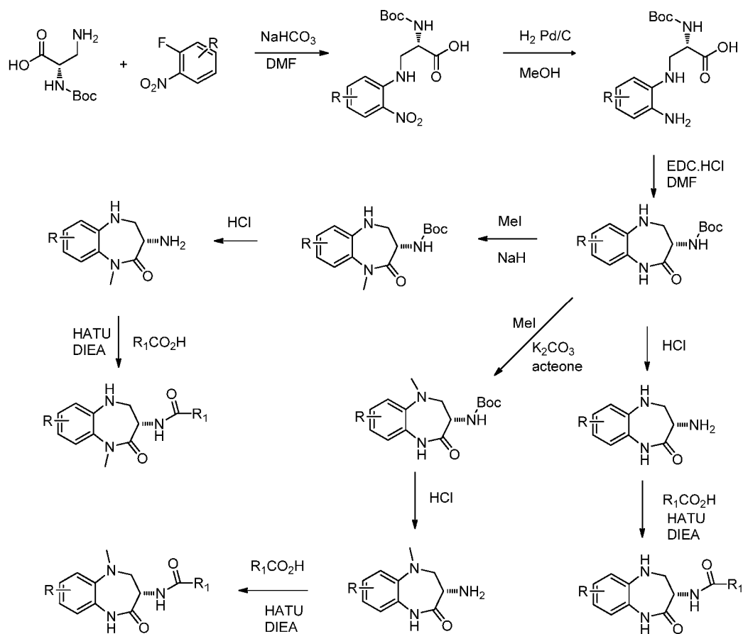
Scheme 3
