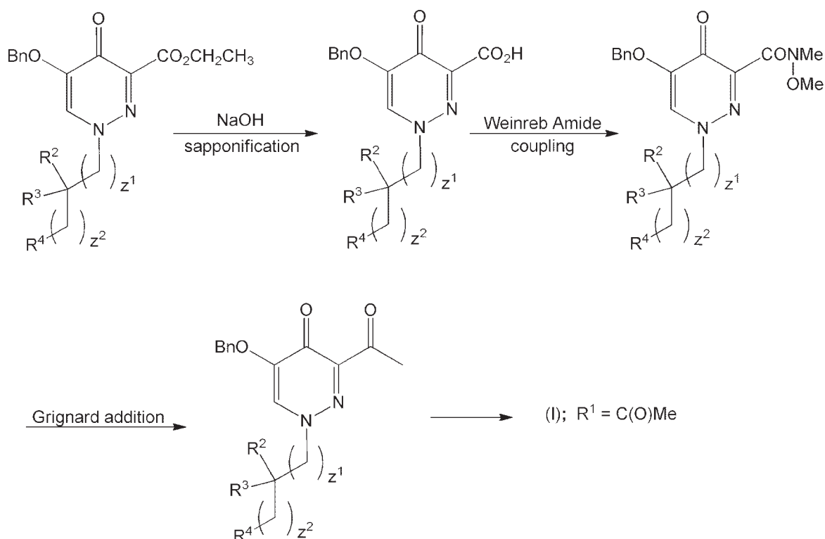
Scheme 6
