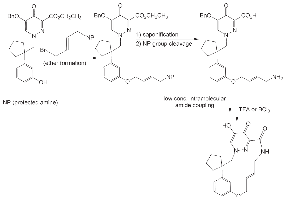
Scheme 10
