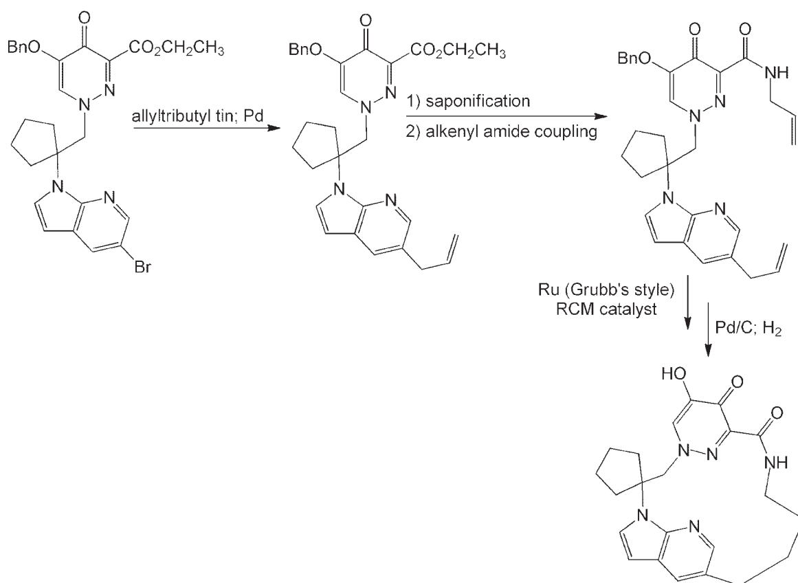
Scheme 9
