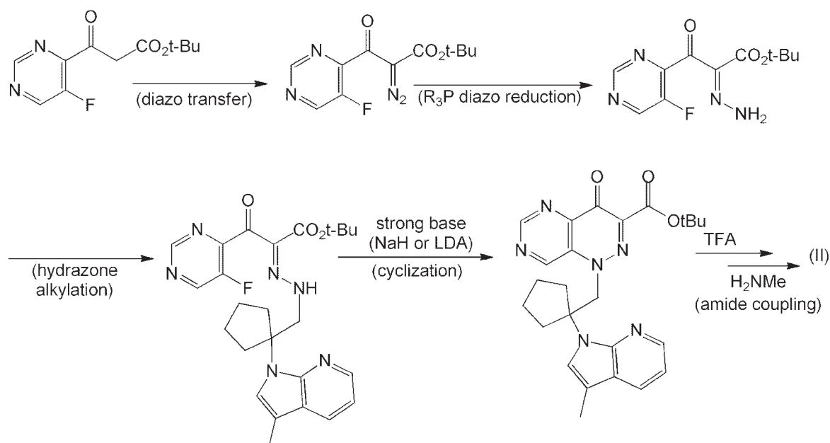
Scheme 11
