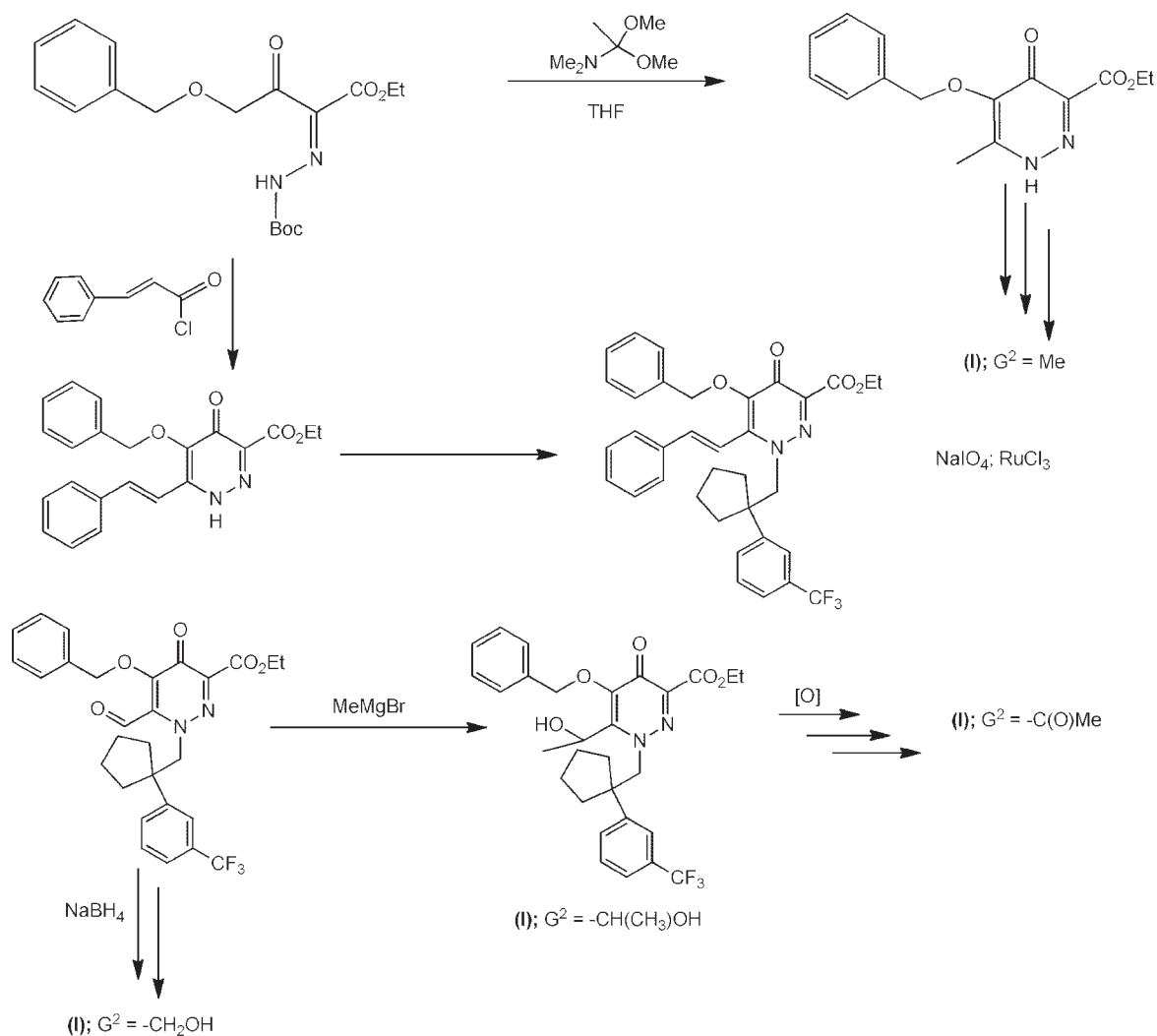
Scheme 7
