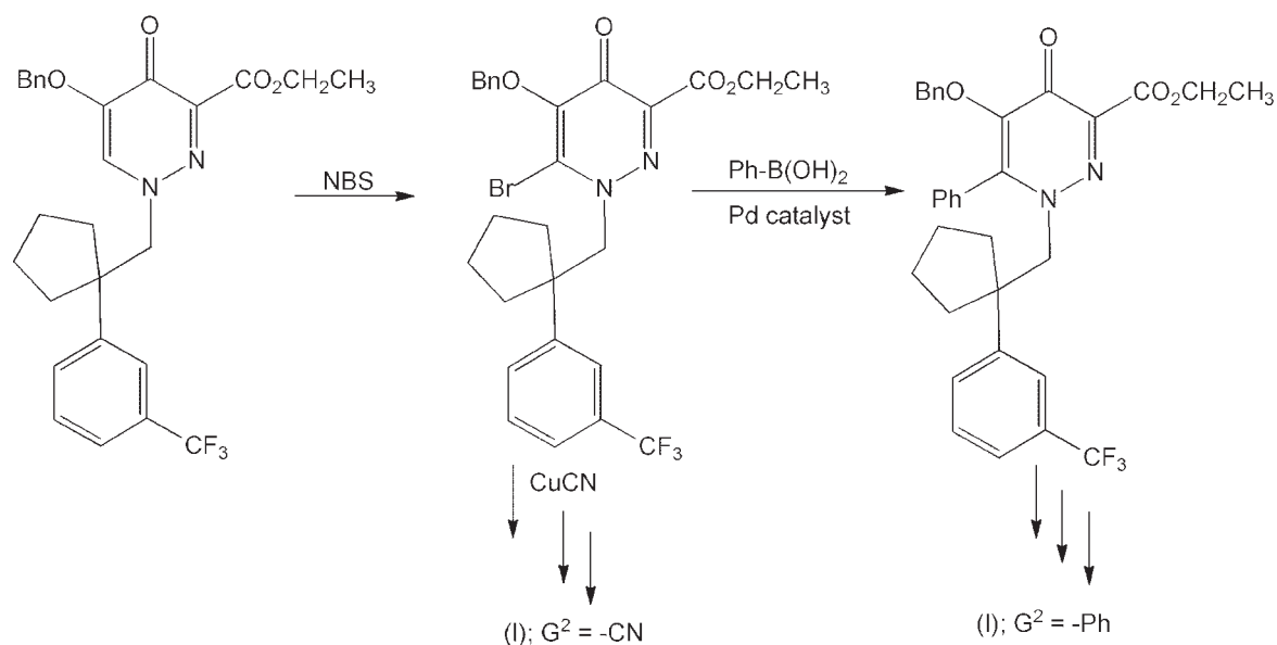
Scheme 8
