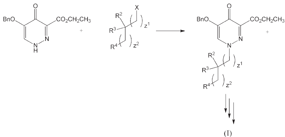
Scheme 4
