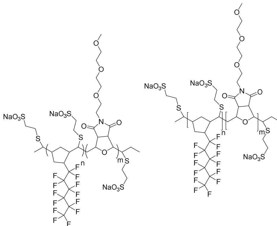
Poly(M8-b-NPF6)-S(CH 2 ) 2 SO 3 Na , Poly(M8-r-NPF6)-S(CH 2 ) 2 SO 3 Na
