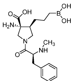
N-methyl phenylalanine AUC = 262
