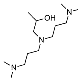
1-[bis-[3-(dimethylamino)]propyl]amino]-2- propanol ("DMAPAP")
