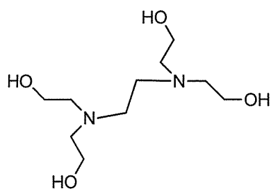
N,N,N',N'-tetrakis(2- hydroxyethyl)ethylenediamine ("THEED")
