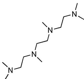
1,1,4,7,10,10-hexamethyltriethylene- tetramine ("HMTETA")
