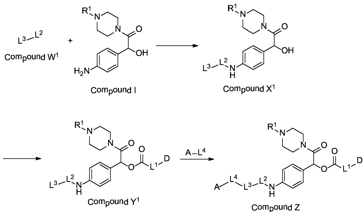
Scheme 5
