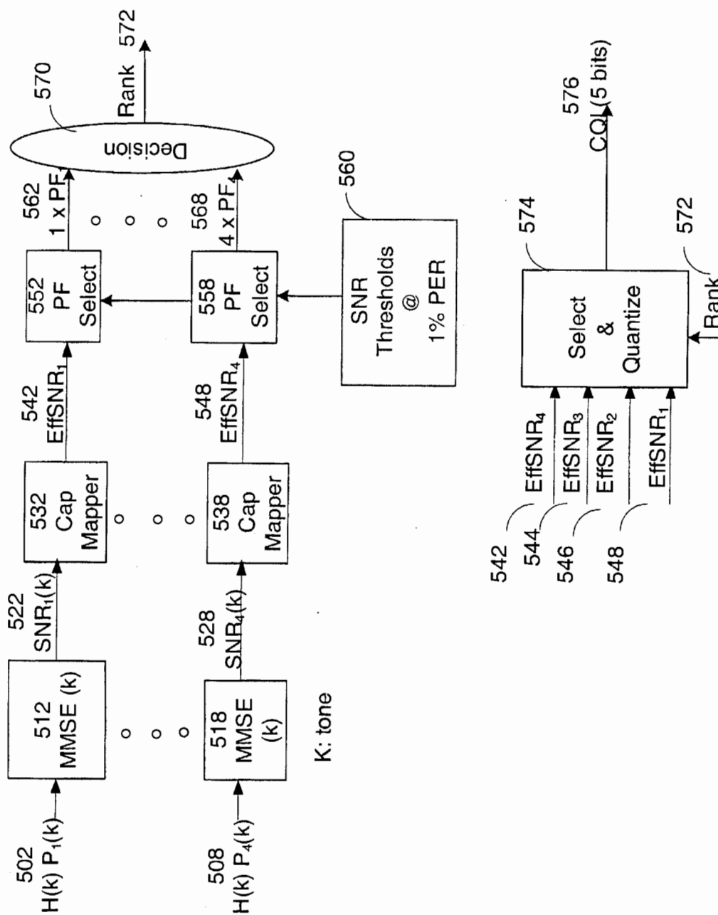
Figure 5: Performance Based Rank Prediction
