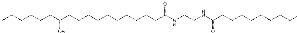
12-HYDROXY-N-[2-(1-OXYDECYL)AMINO]ETHYLOCTADECANAMIDE
