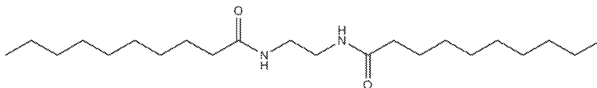
N,N'-ETHANE-1,2-DIYLBIS(DECANAMIDE)
