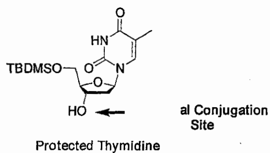
Representative Nucleosides
