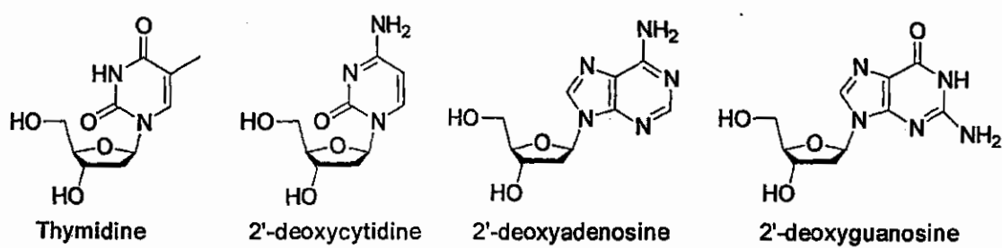
Representative Nucleosides
