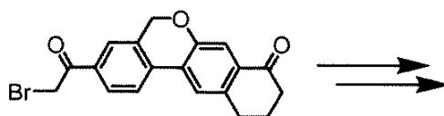
3-(2-bromoacetyl)-10,11-dihydro-5H-dibenzo[c,g]chromen-8(9H)-one
