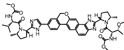
methyl [(2S)-1-[(2S,5S)-2-[5-(2-[(2S,5S)-1-[N-(methoxycarbonyl)-O-methyl-L-threonyl]-5-methylpyrrolidin-2-yl]-1,11-dihydroisochromeno[4',3':6,7]naphtho[1,2-d]imidazol-9-yl)-1H-imidazol-2-yl]-5-methylpyrrolidin-1-yl]-3-methyl-1-oxobutan-2-yl]carbamate
