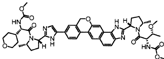
methyl [(1S)-2-[(2S,5S)-2-(5-{2-[(2S,5S)-1-[(2S,3R)-3-methoxy-2-[(methoxycarbonyl)amino]butanoyl]-5-methylpyrrolidin-2-yl]-1,11-dihydroisochromeno[4',3':6,7]naphtho[1,2-d]imidazol-9-yl]-1H-imidazol-2-yl)-5-methylpyrrolidin-1-yl]-2-oxo-1-(tetrahydro-2H-pyran-4-yl)ethyl]carbamate
