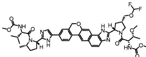
methyl [(2S,3R)-1-[(2S,4S)-4-[(difluoromethoxy)methyl]-2-[9-(2-[(2S,5S)-1-[N-(methoxycarbonyl)-L-valyl]-5-methylpyrrolidin-2-yl]-1H-imidazol-5-yl)-1,11-dihydroisochromeno[4',3':6,7]naphtho[1,2-d]imidazol-2-yl]pyrrolidin-1-yl]-3-methoxy-1-oxobutan-2-yl]carbamate
