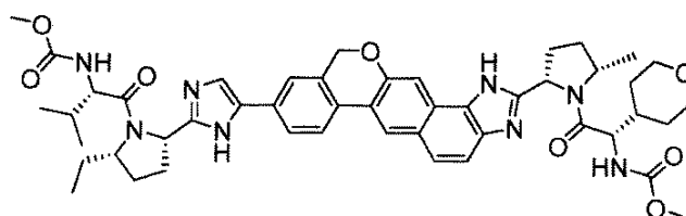
Methyl[(1S)-2-[(2S,5S)-2-(9-{2-[(2S,5S)-5-ethyl-1-[(2S)-2[(methoxycarbonyl)amino]-3-methylbutanoyl]pyrrolidin-2-yl]-1H-imidazol-5-yl]-1,1-dihydroisochromeno [4',3':6,7]naphtho[1,2-d]imidazol-2-yl)-5-methylpyrrolidin-1-yl]-2-oxo-1(tetrahydro-2H-pyran-4-yl)ethyl]carbamate
