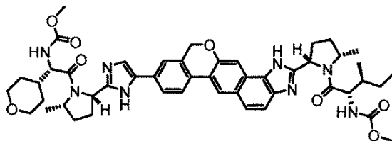
methyl [(1S)-2-[(2S,5S)-2-(5-{2-[(2S,5S)-1-[(2S,3S)-2-[(methoxycarbonyl)amino]-3-methylpentanoyl]-5-methylpyrrolidin-2-yl]-1,11-dihydroisochromeno[4',3':6,7]naphtho[1,2-d]imidazol-9-yl]-1H-imidazol-2-yl)-5-methylpyrrolidin-1-yl]-2-oxo-1-(tetrahydro-2H-pyran-4-yl)ethyl]carbamate
