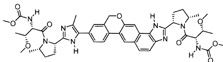
methyl [(2S,3R)-3-methoxy-1-{(2S,5S)-2-[9-(2-{(2S,5S)-1-[N-(methoxycarbonyl)-O-methyl-L-threonyl]-5-methylpyrrolidin-2-yl)-4-methyl-1H-imidazol-5-yl]-1,11-dihydroisochromeno[4',3':6,7]naphtho[1,2-d]imidazol-2-yl]-5-methylpyrrolidin-1-yl}-1-oxobutan-2-yl]carbamate
