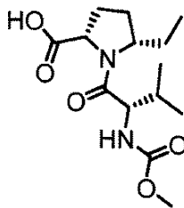
(2S,5S)-5-ethyl-1-((S)-2-(methoxycarbonylamino)-3-methylbutanoyl)pyrrolidine-2-carboxylic acid
