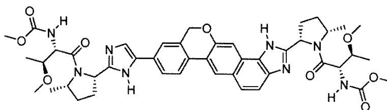
methyl [(2S,3S)-3-methoxy-1-[(2S,5S)-2-[9-(2-[(2S,5S)-1-[N-(methoxycarbonyl)-O-methyl-L-allothreonyl]-5-methylpyrrolidin-2-yl]-1H-imidazol-5-yl)-1,11-dihydroisochromeno[4',3':6,7]naphtho[1,2-d]imidazol-2-yl]-5-methylpyrrolidin-1-yl]-1-oxobutan-2-yl]carbamate
