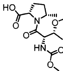
(2S,5S)-1-((2S,3R)-3-methoxy-2-(methoxycarbonylamino)butanoyl)-5-methylpyrrolidine-2-carboxylic acid
