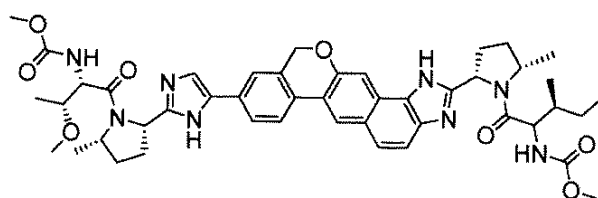
methyl{(3S)-1-[(2S,5S)-2-(9-{2-[(2S,5S)-1-[(2S,3R)-3-methoxy-2-[(methoxycarbonyl) amino]butanoyl)-5-methylpyrrolidin-2-yl]-1H-imidazol-5-yl}-1,11-dihydroisochromeno[4',3':6,7]naphtho[1,2-d]imidazol-2-yl)-5-methylpyrrolidin-1-yl]-3-methyl-1-oxopentan-2-yl}carbamate
