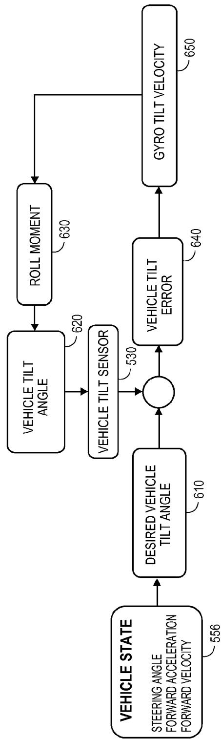
Control System Diagram
