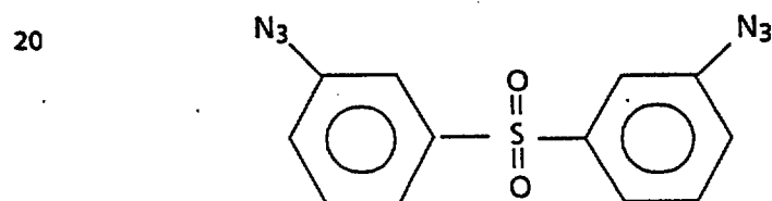
25 m-Azidophenyl Sulfone
