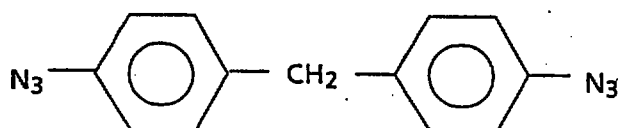
4,4'-Diazido diphenyl methane
