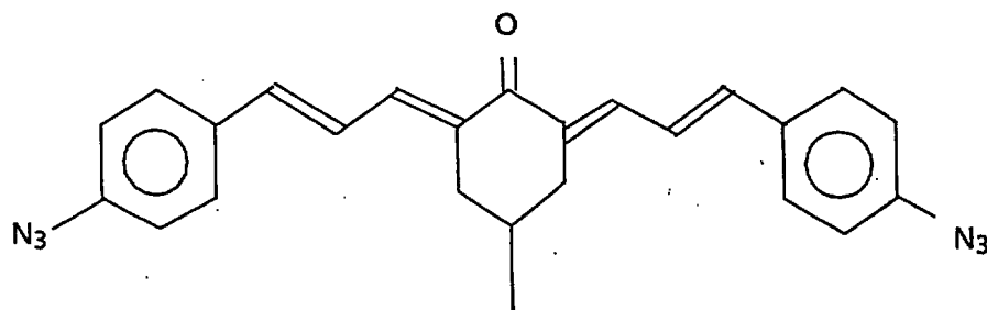
2,6-Bis[3-(4-azidophenyl)-2-propenylidene]-4-methylcyclohexanone
