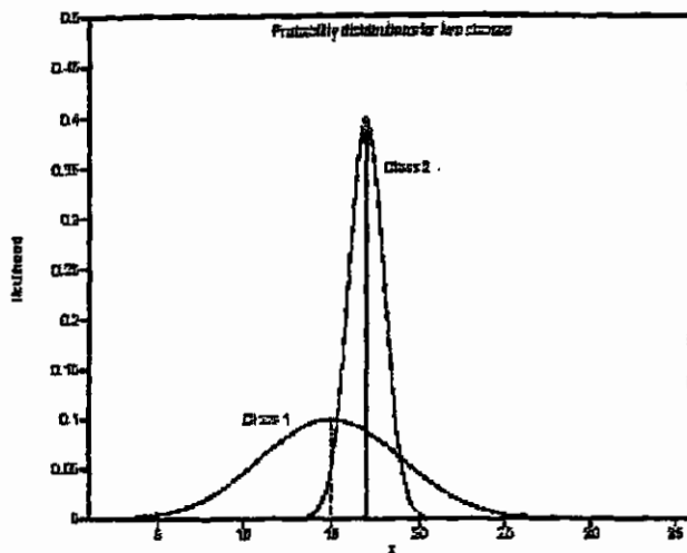
Figur 2 Two classes were the Bayes classifier uses quadratic decision surfaces.
