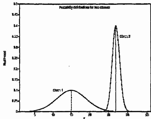
Figur 2 Two classes were the Bayes classifier uses quadratic decision surfaces.
