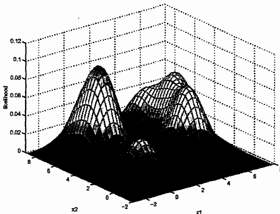
Figure 5: Likely Hood
