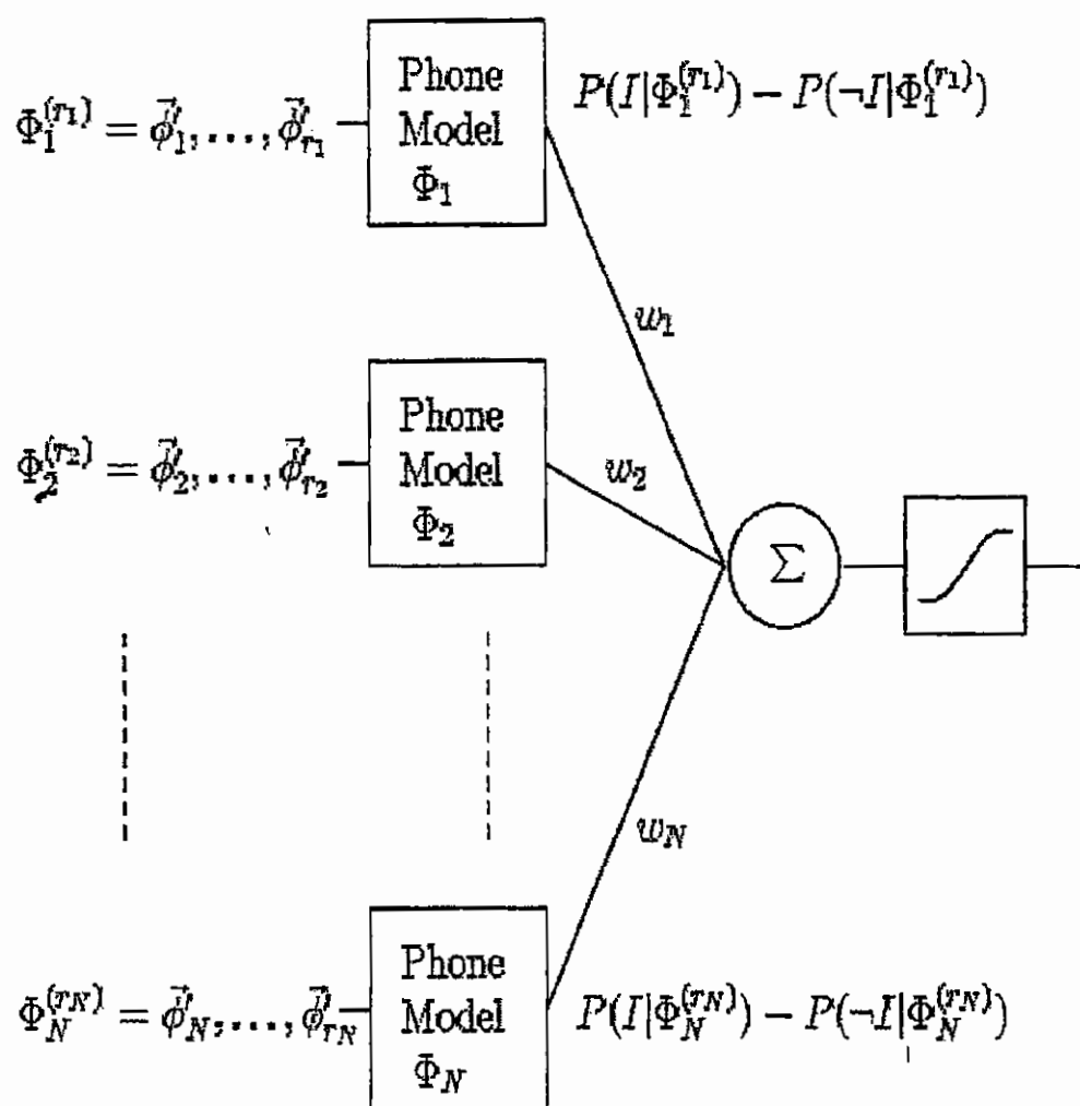
Figure: 2 A super classifier
