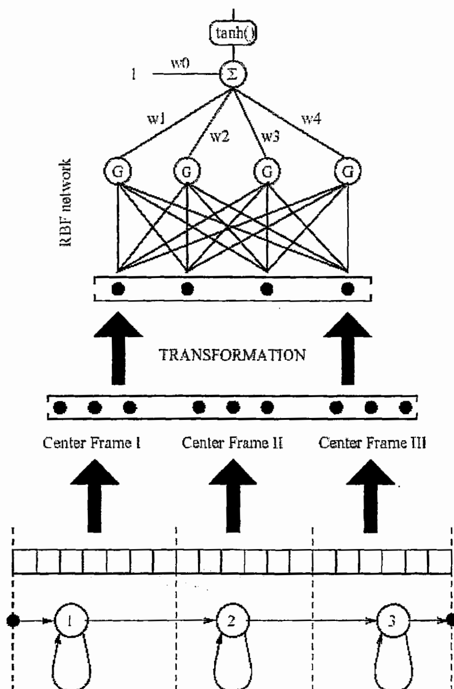
Figur 7: RBF network
