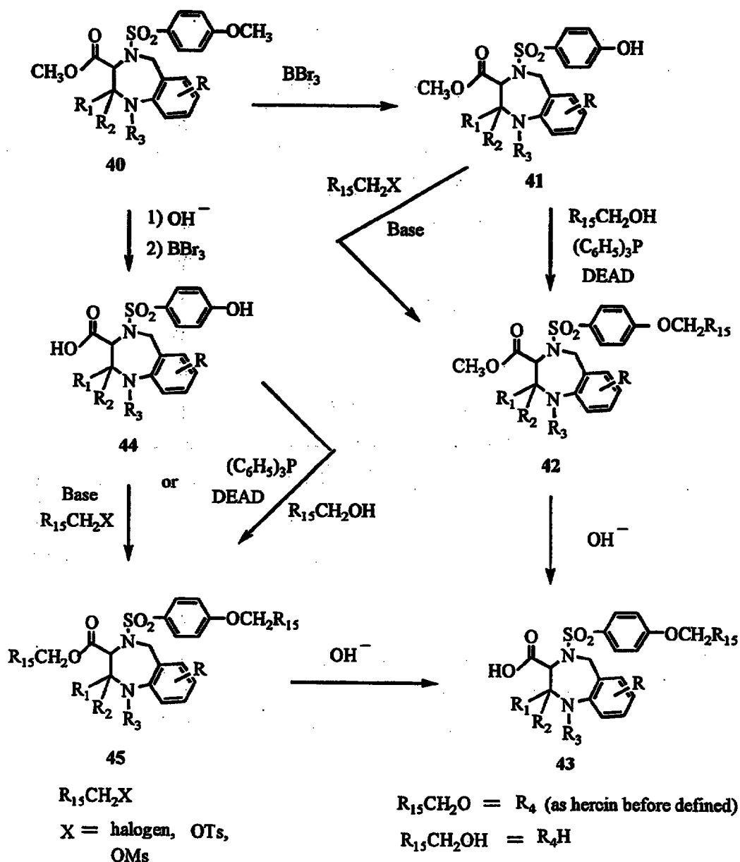
Scheme 8
