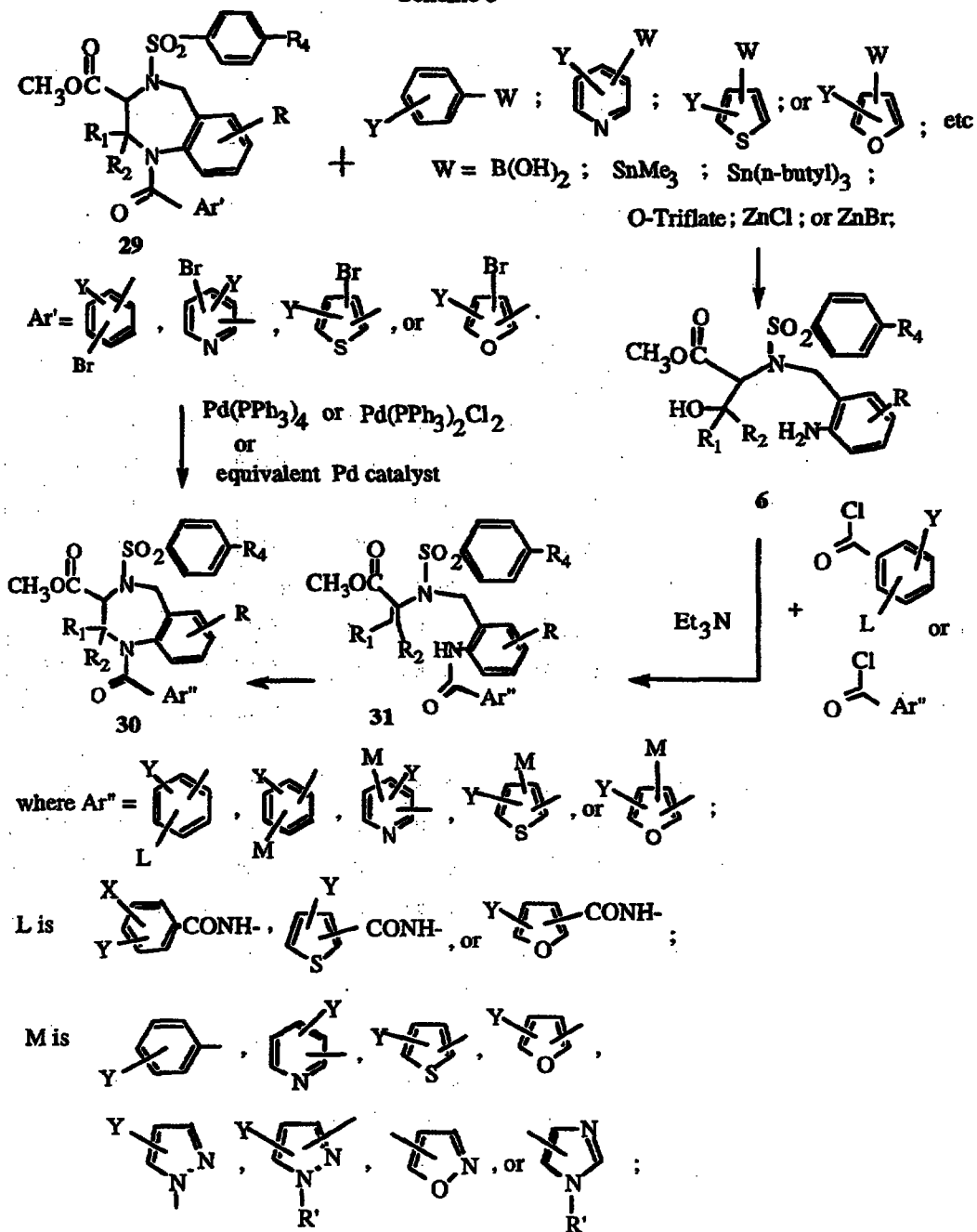
Scheme 6
