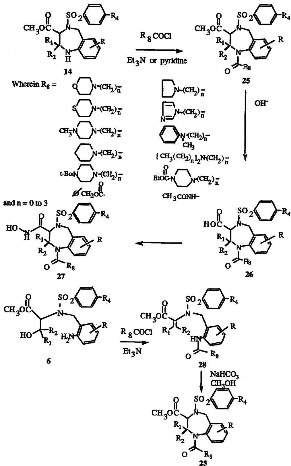
Scheme 5
