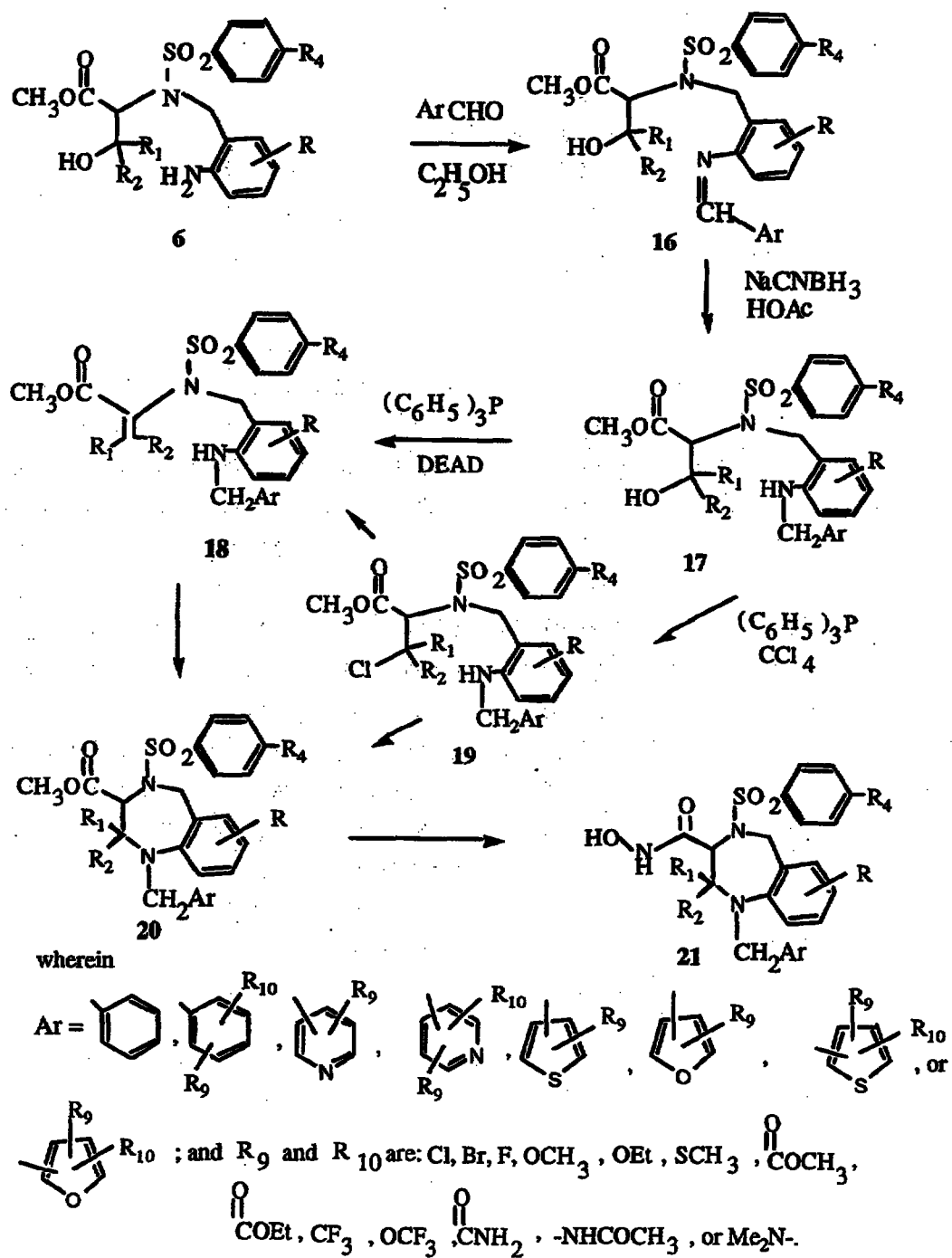
Scheme 3
