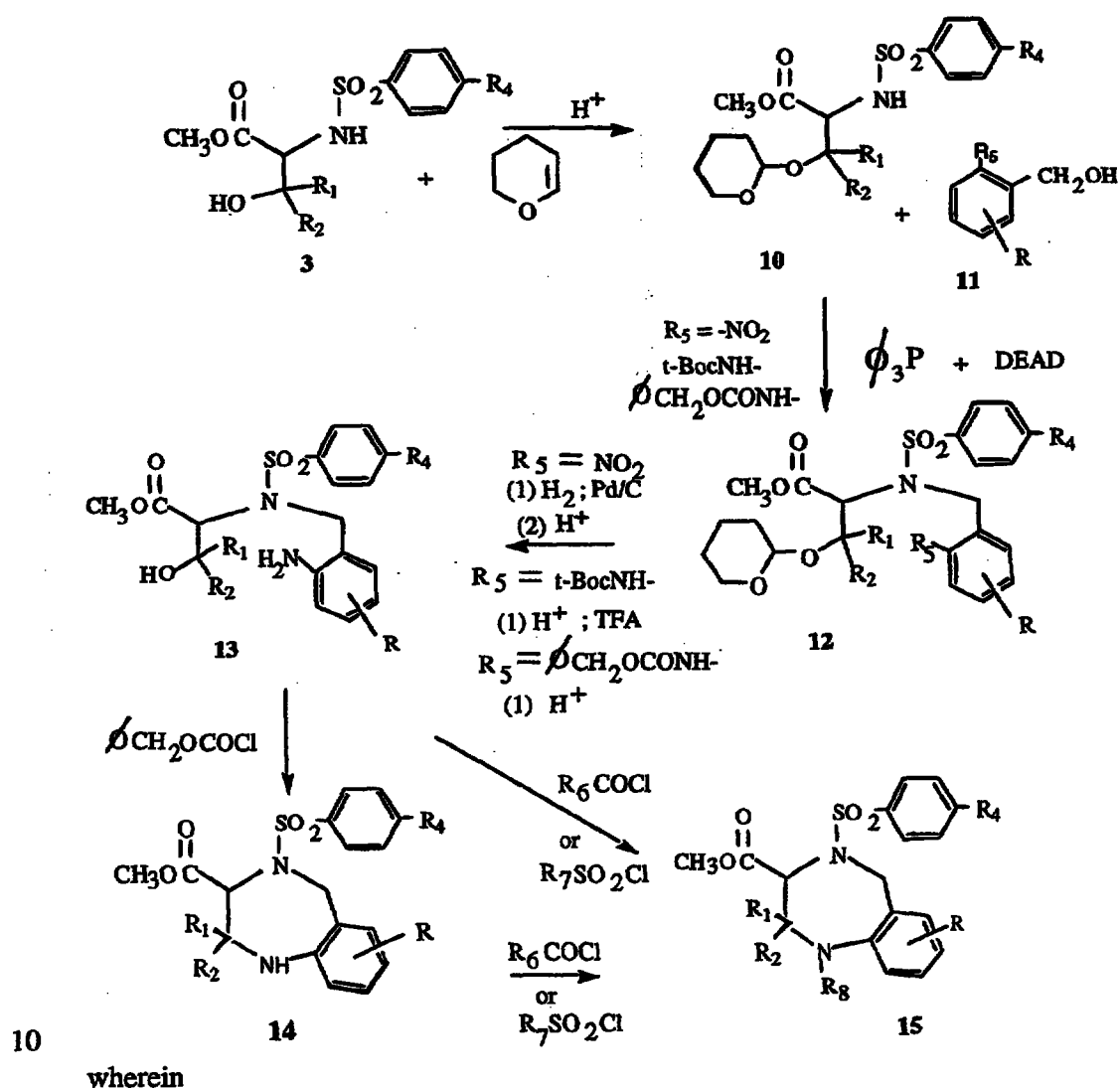
Scheme 2
