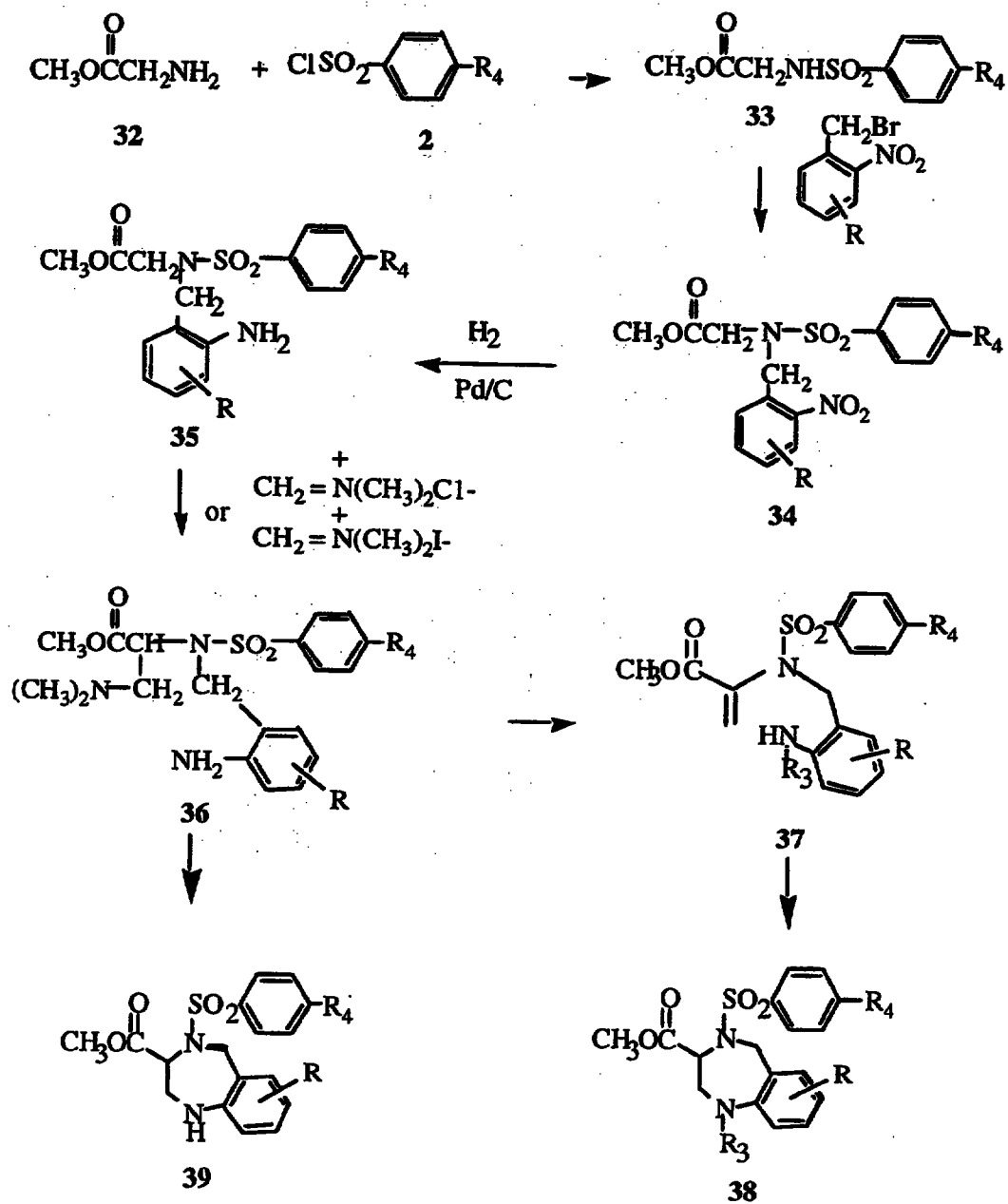
Scheme 7
