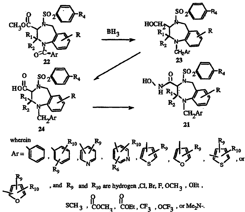
Scheme 4
