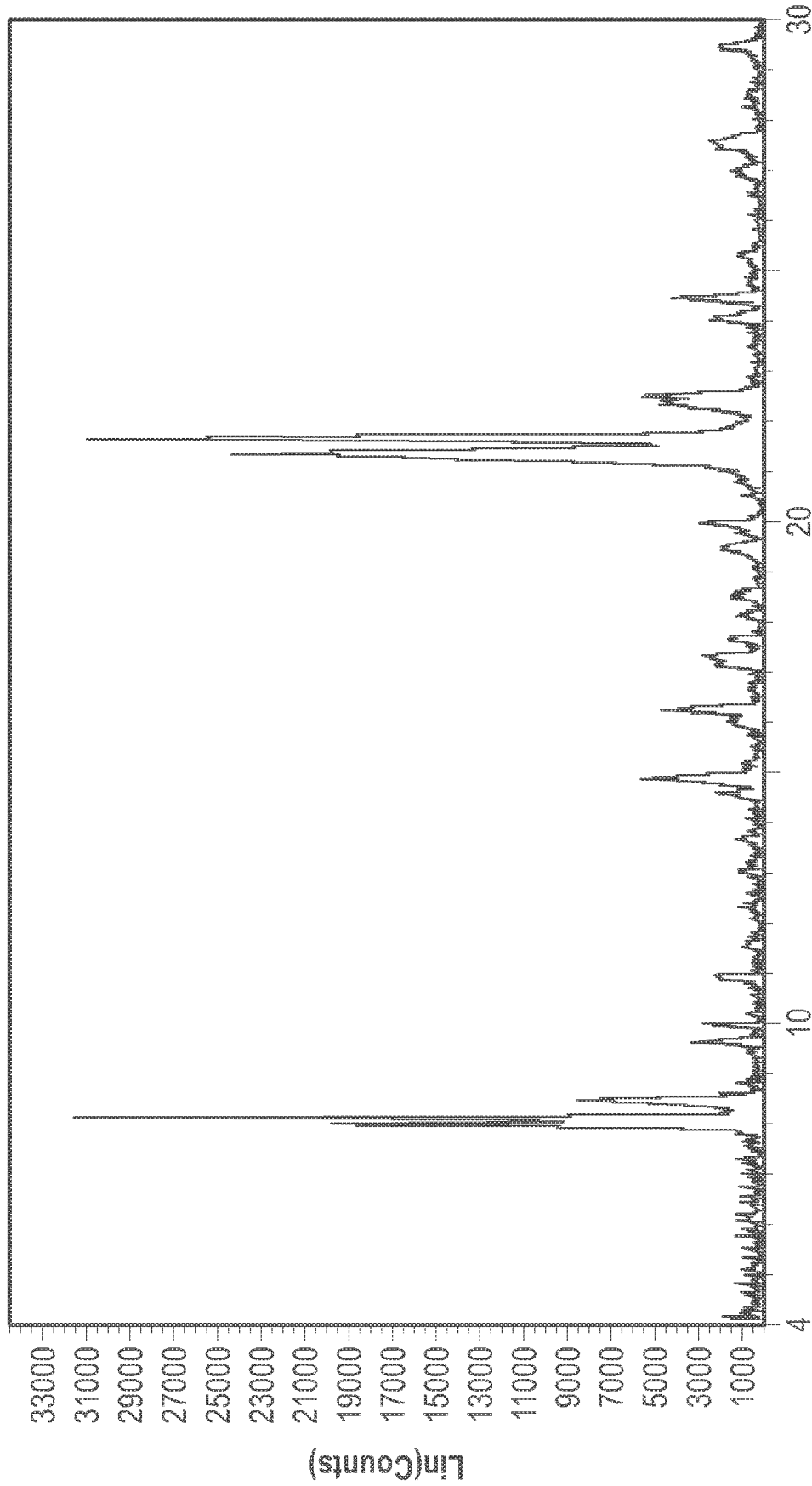
2-Theta-Scale FIG. 22
