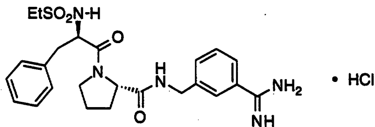
\text{EtSO}_2\text{-D-Phe-Pro-m-NHCH}_2\text{-C}_6\text{H}_4\text{C(=NH)NH}_2 \cdot \text{HCl}
