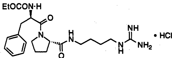
EtOCO-D-Phe-Pro-Agm·HCl
