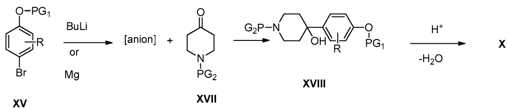
Synthetic scheme 4b:
