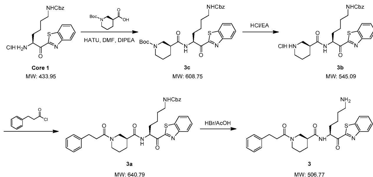
Scheme 10
