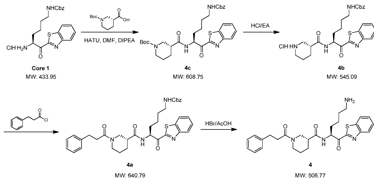
Scheme 11
