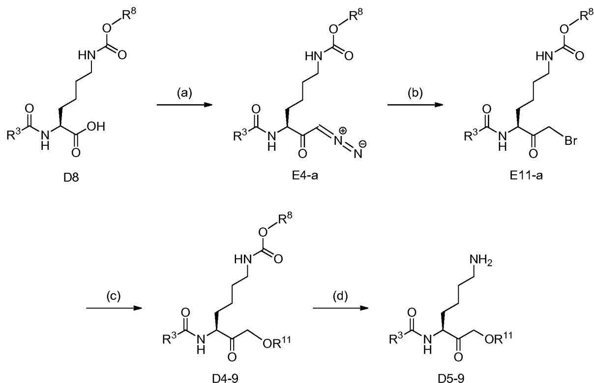
Scheme 6
