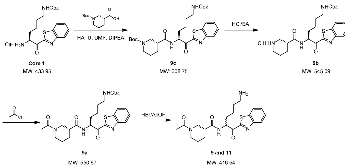
Scheme 14
