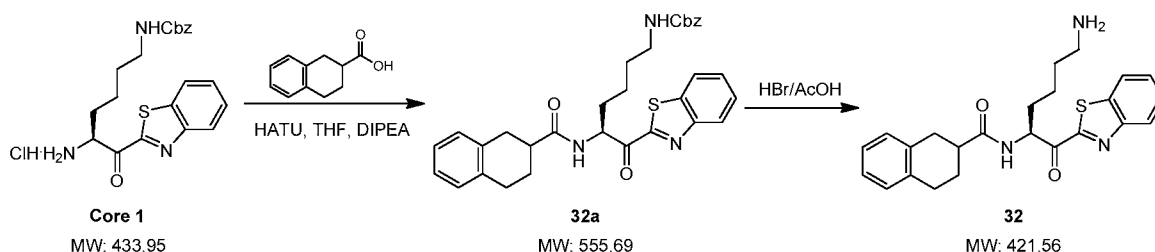
Scheme 26
