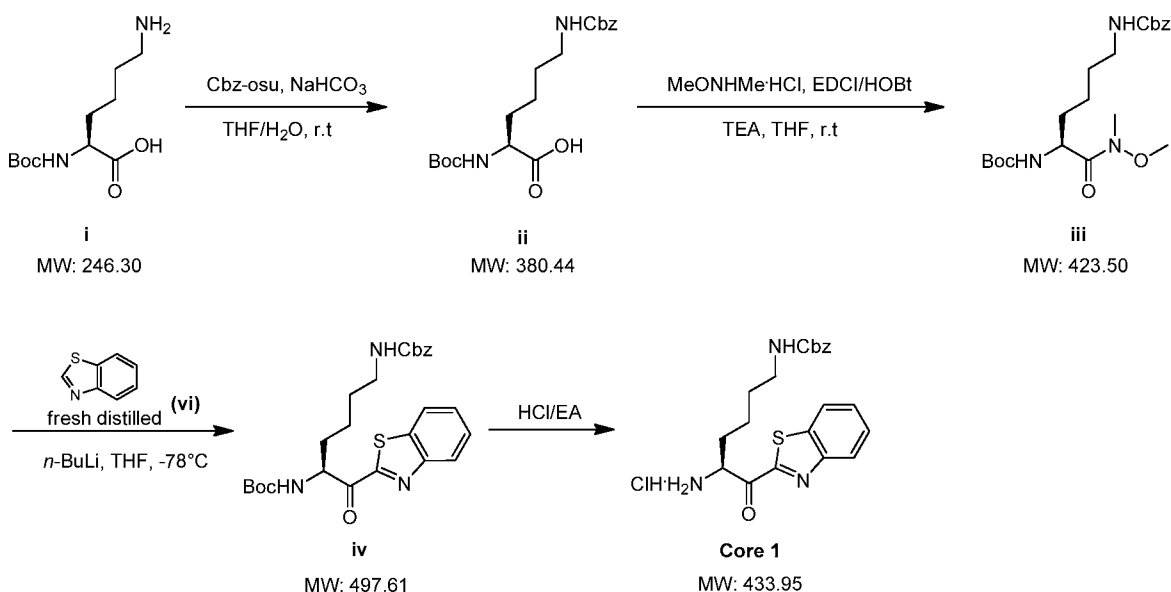
Scheme 7
