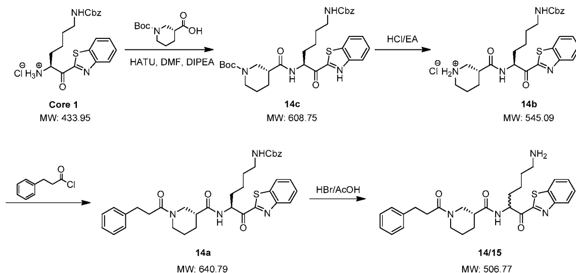
Scheme 17
