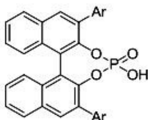
Formula VII
