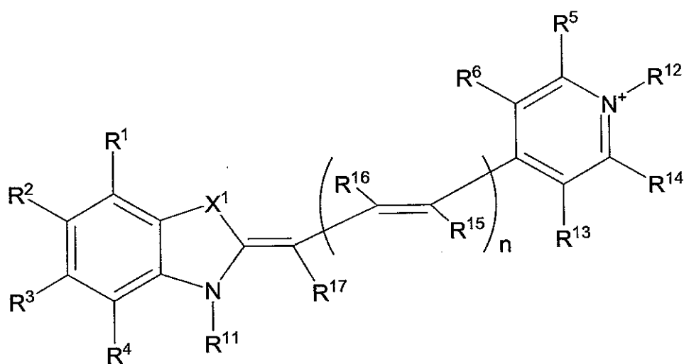
[Chemical Formula 6]
