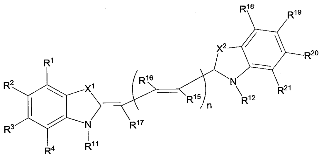
[Chemical Formula 7]
