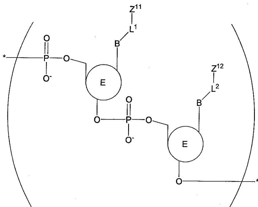
[Chemical Formula 3]
