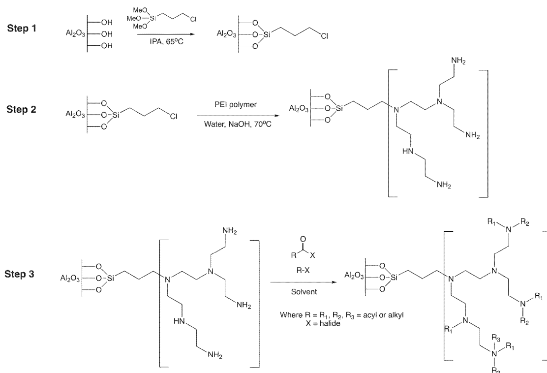
Scheme 1: Synthesis of the functionalised alumina substrate (any counter ions omitted for clarity).
