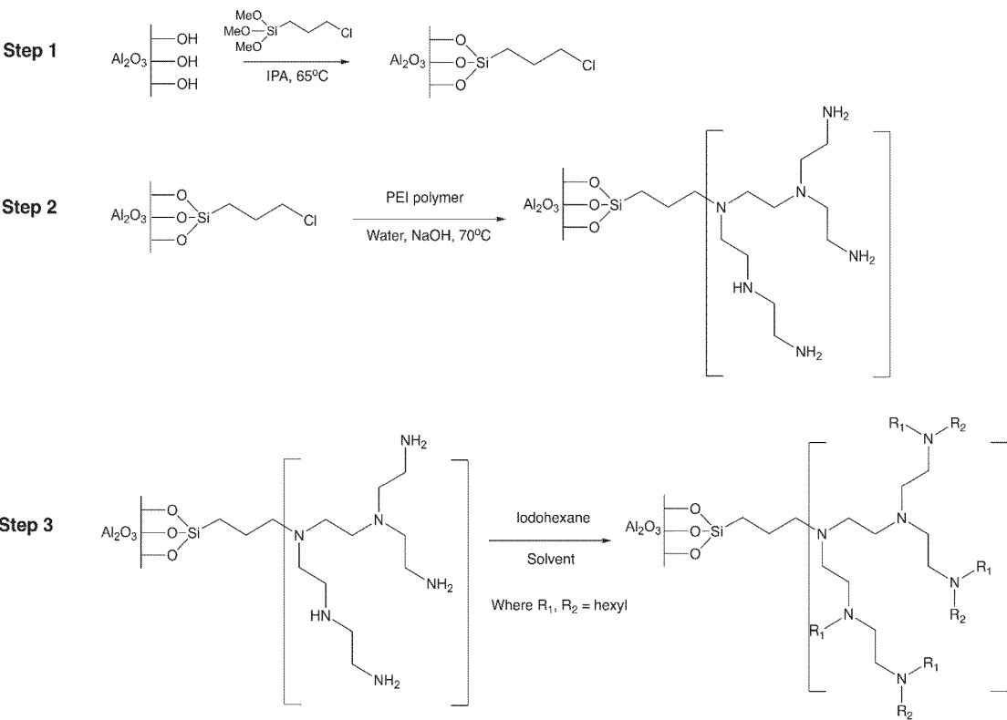
Scheme 2: Synthesis of the functionalised alumina substrate (any counter ions omitted for clarity).
