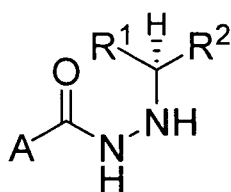
Formula S -XIV
