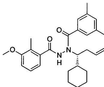
(R)-3,5-Dimethylbenzoic acid N-(1-cyclohexyl-but-3-enyl)-N'-(3-methoxy-2-methylbenzoyl)-hydrazide
