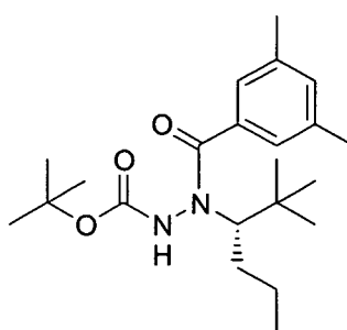
(S)-N'-(1- tert -Butyl-butyl)-N'-(3,5-dimethyl-benzoyl)-hydrazinecarboxylic acid tert -butyl ester
