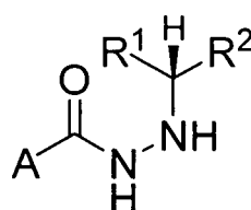
Formula R -XIV
