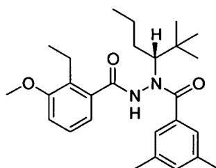
( R )-3,5-Dimethyl-benzoic acid N-(1- tert -butyl-butyl)-N'-(2-ethyl-3-methoxy-benzoyl)-hydrazide
