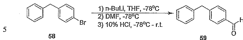
Scheme 5.
