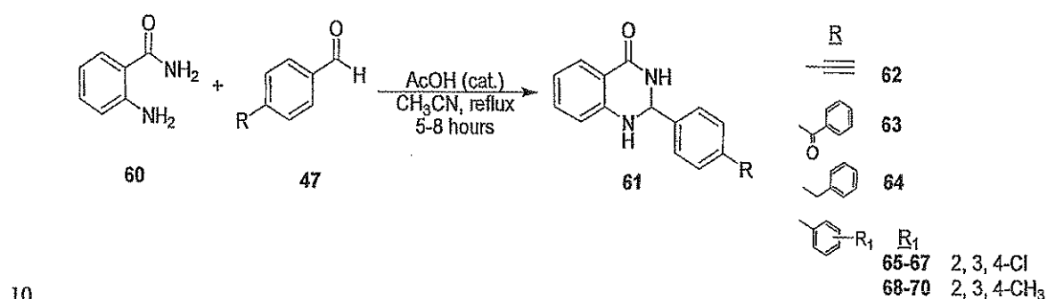
Scheme 6. Synthesis of second generation analogues 62-70.
