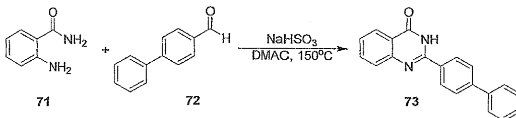
Scheme 7. Synthesis of unsaturated quinazolinones
