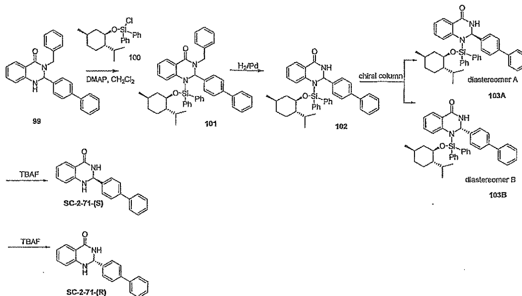
Scheme 12. Chiral resolution of SC-2-71.
