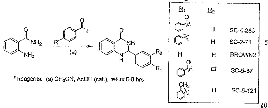
Scheme 1. Synthetic route for SC-2-71 and analogues.
