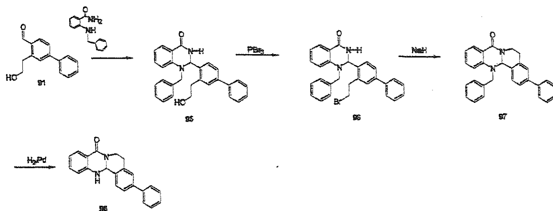
Scheme 11. Synthesis of rigid analogues (amide).
