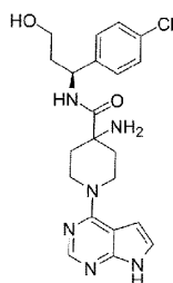
Compound [I]
