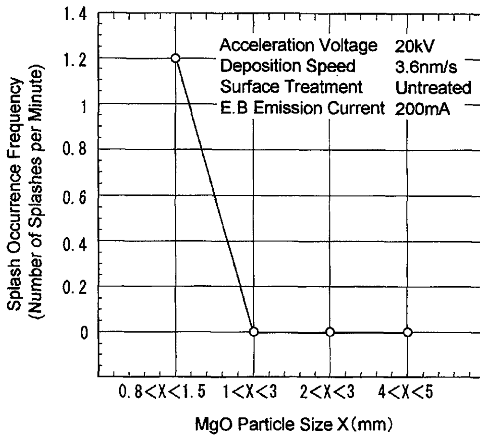
Relationship between Splash Occurrence Frequency and MgO Particle Size
