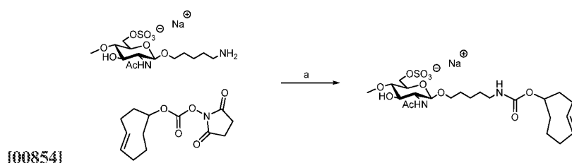
[00855] Synthetic Scheme 3-4
