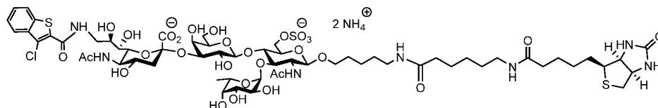
[001094] S212-biotin
