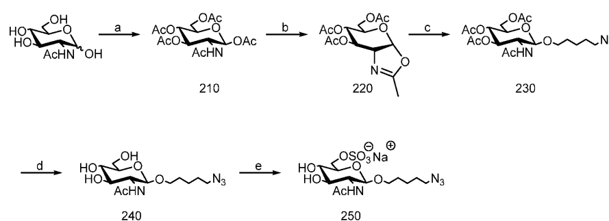
Scheme 10-10
