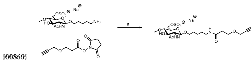
[00859] Synthetic Scheme 3-6
