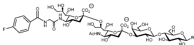
[00940] Compound D110
