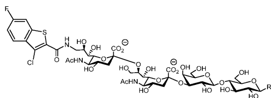
[00958] Compound D212
