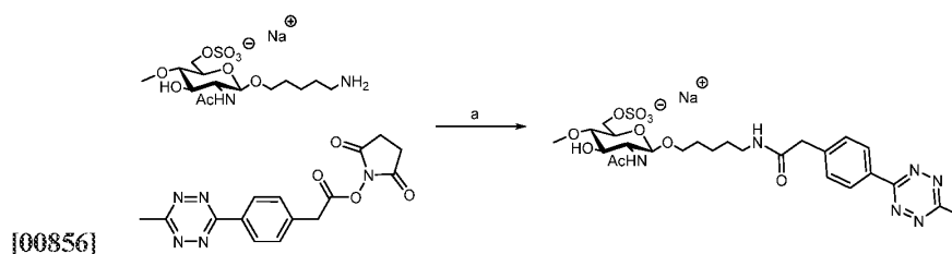
[00857] Synthetic Scheme 3-5
