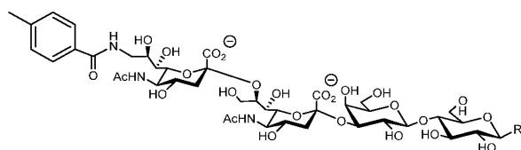
[00960] Compound D214
