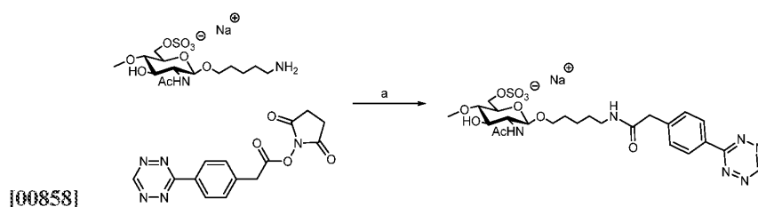
[00859] Synthetic Scheme 3-6
