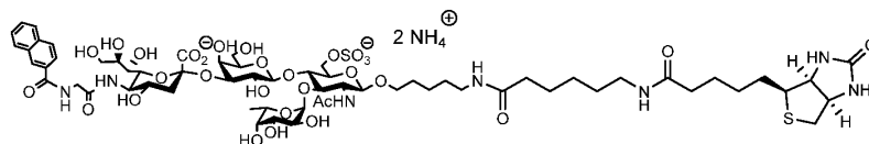
[001090] S102-biotin
