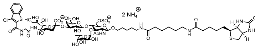
[001094] S212-biotin
