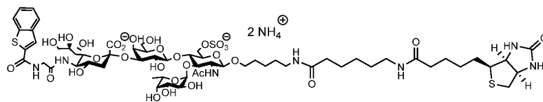
[001093] S112-biotin
