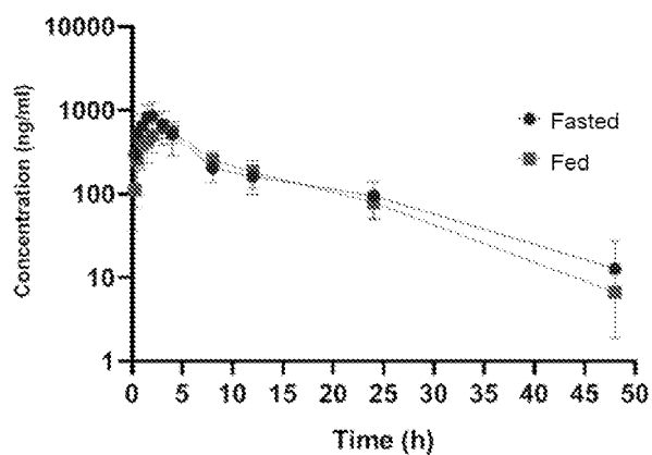
Ezogabine Plasma Concentrations as a Function of Time Following Oral Administration of a Single 400 mg Dose of Ezogabine (as 2.0 g of the Formulation of Example 12) Under Fasted or Fed Conditions
