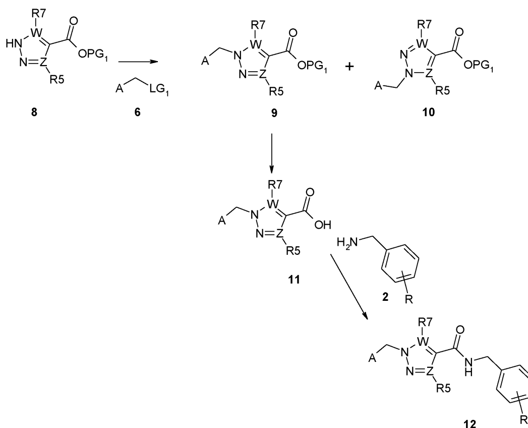
Scheme 2b
