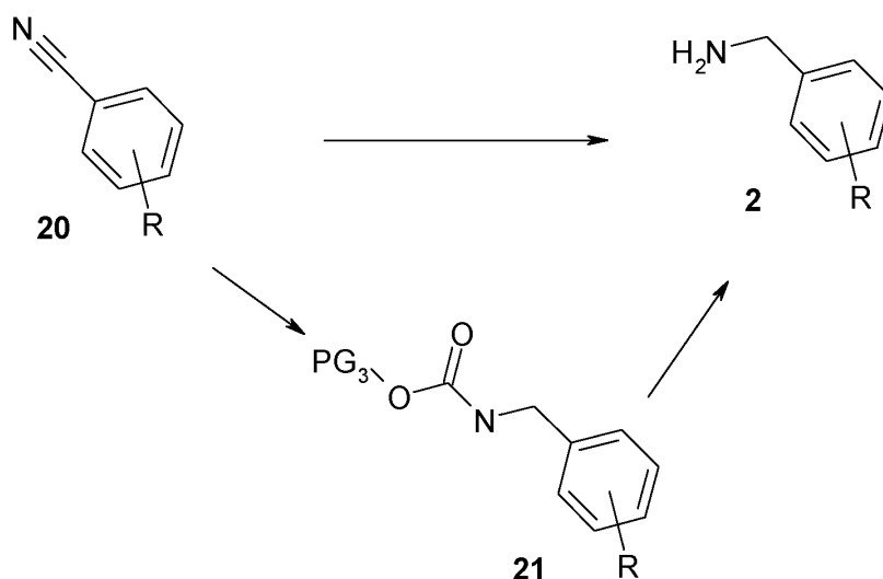
Scheme 4
