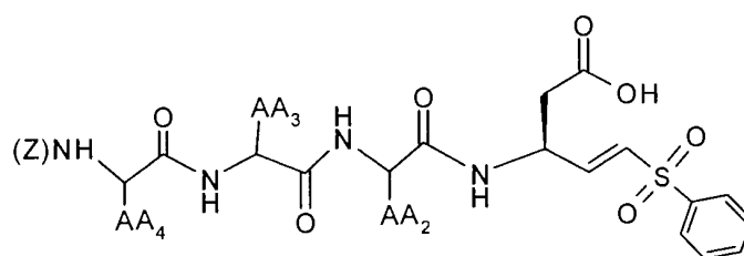
Formula 1f
