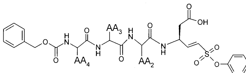
Formula 1g
