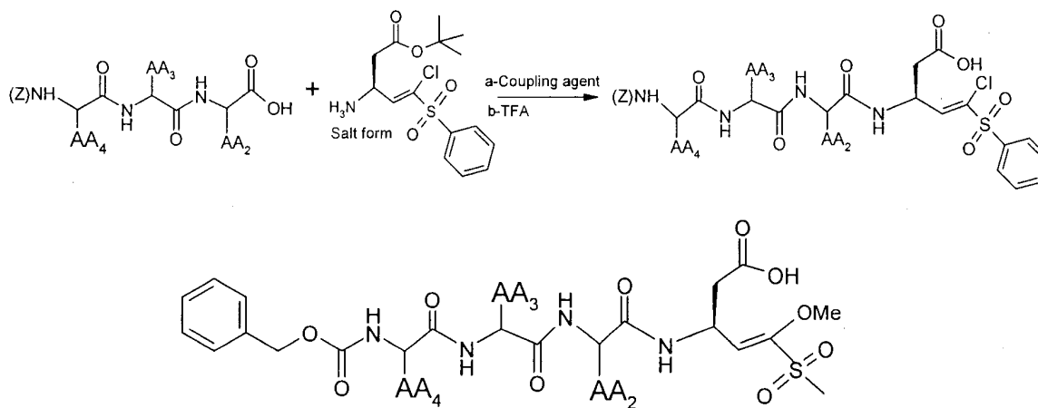
Formula 1c
