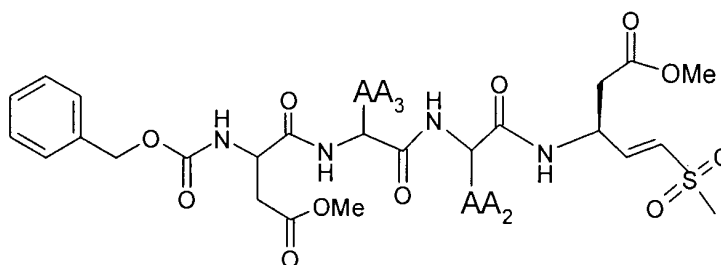
Formula 1i
