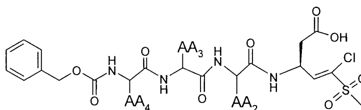
Formula 1a
