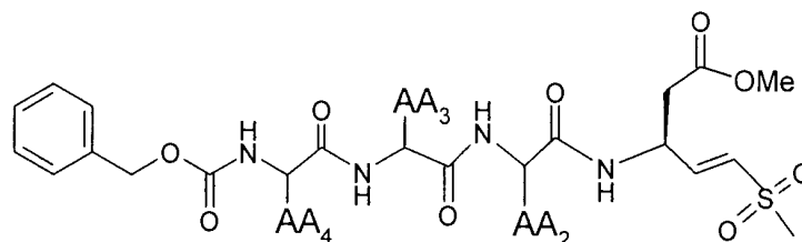
Formula 1d
