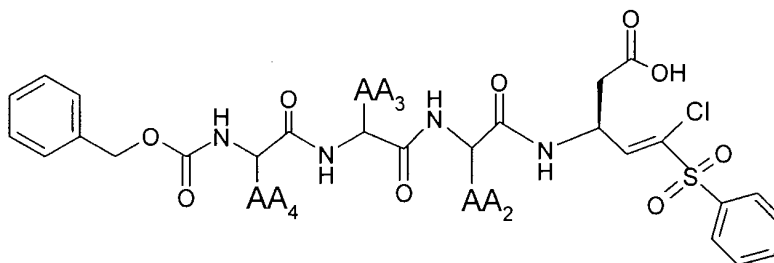
Formula 1b
