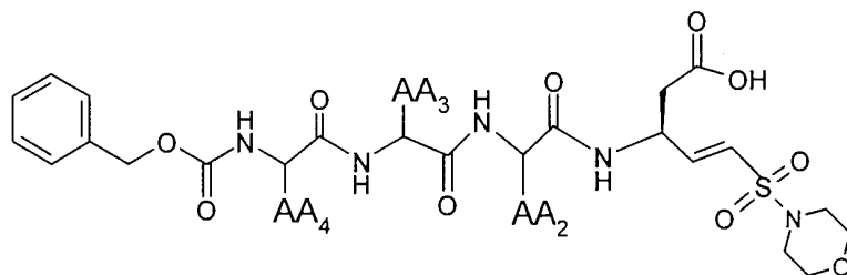
Formula 1h
