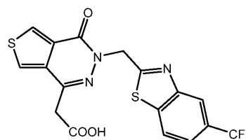
Compound B
