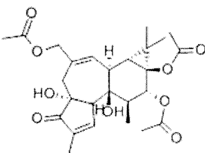
Phorbol 12,13,20- Triacetate
