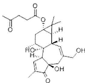
12-Deoxyphorbol 13-Angelate
