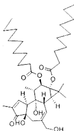
Phorbol 12,13- Didecanoate
