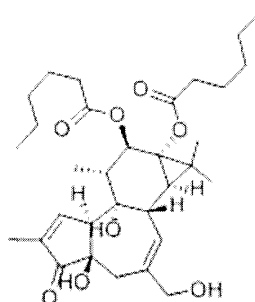
Phorbol 12,13- Dihexanoate
