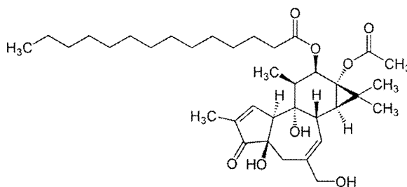
Phorbol 12- Myristate-13- Acetate (also known as TPA or PMA)
