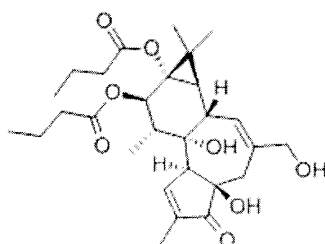
Phorbol 12,13- Dibutyrate
