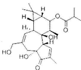
12-Deoxyphorbol 13-Isobutyrate
