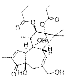
Phorbol 12,13- Dipropionate
