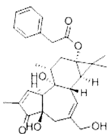
12-Deoxyphorbol 13-Phenylacetate
