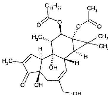
Formula II.
