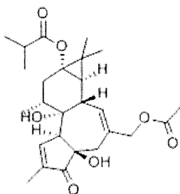
12-Deoxyphorbol 13-Isobutyrate-20- Acetate
