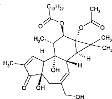
Formula II
