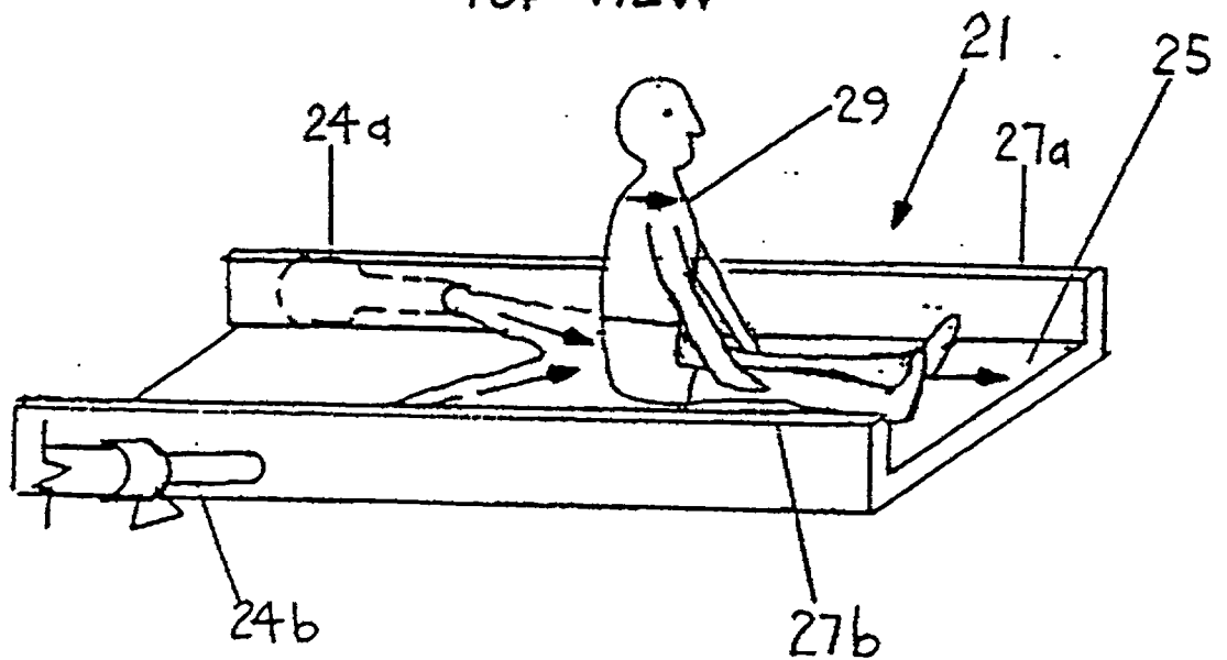
FIG 4C PERSPECTIVE VIEW
