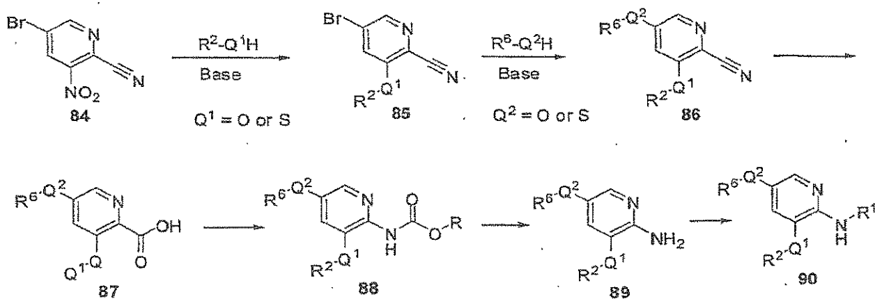
Scheme W
