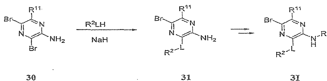
Scheme K
