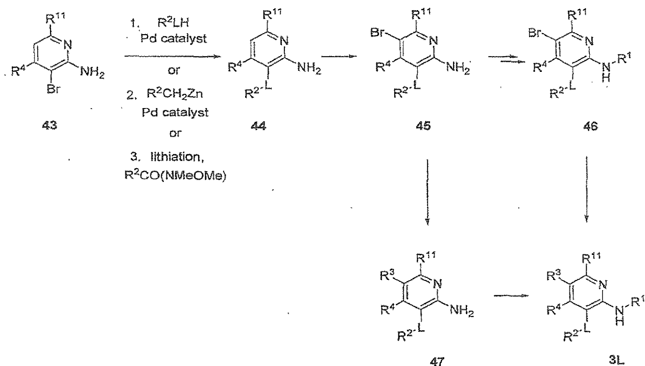
Scheme O
