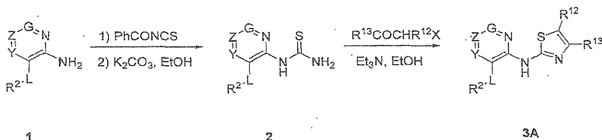
Scheme A
