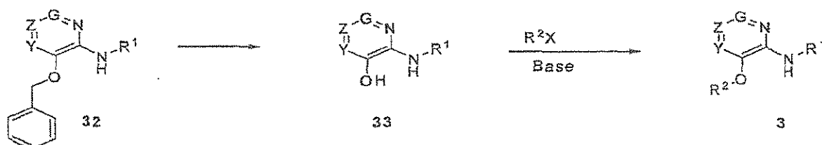
Scheme L
