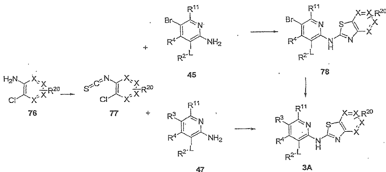
Scheme U
