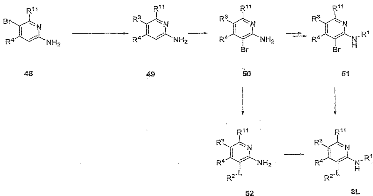
Scheme P
