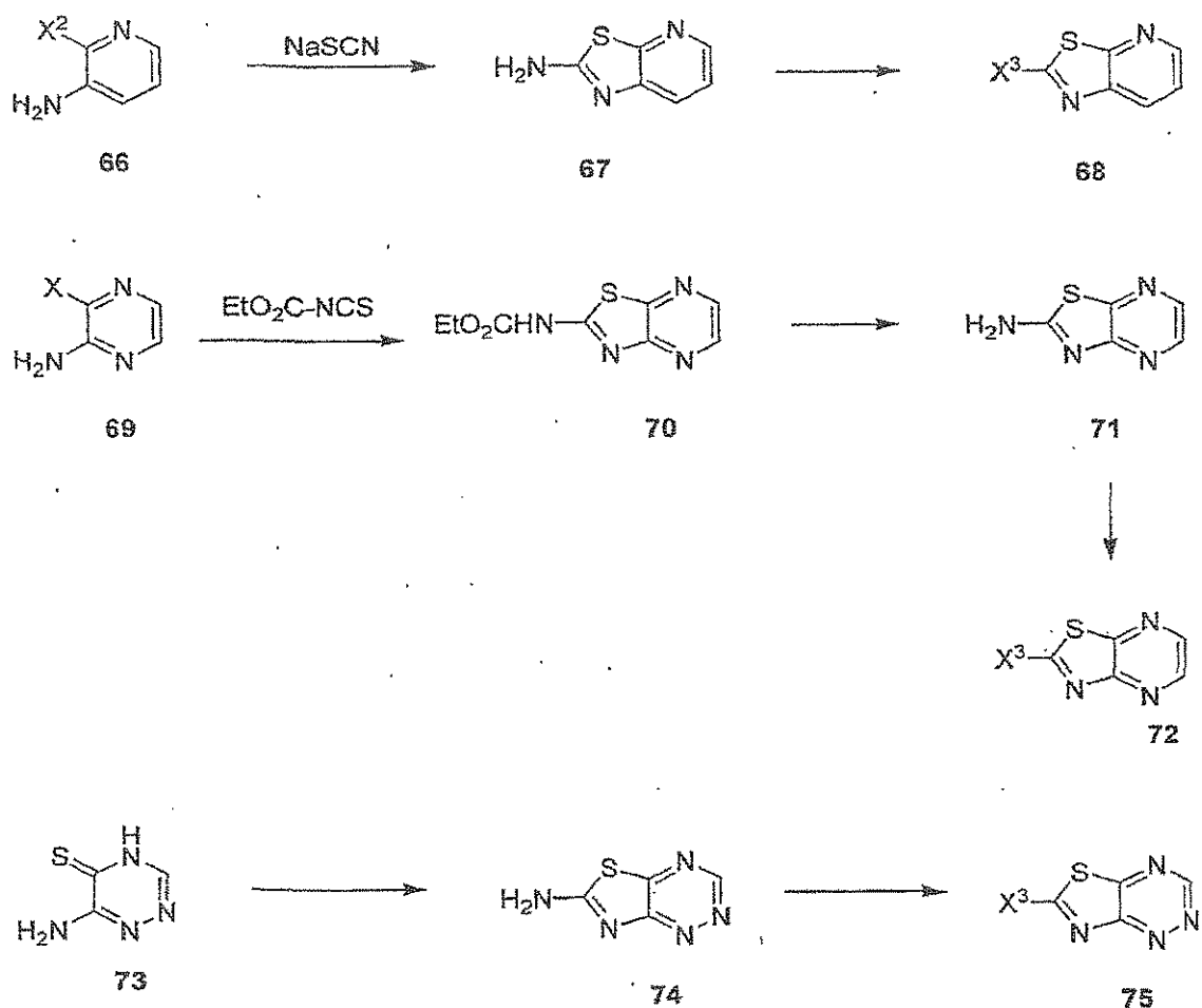
Scheme T
