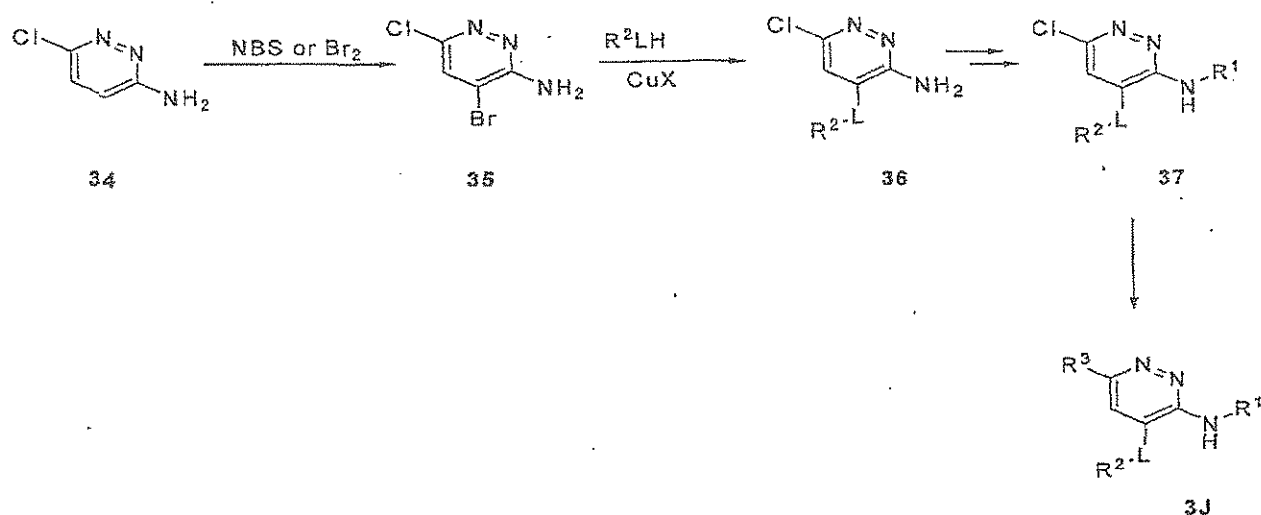
Scheme M
