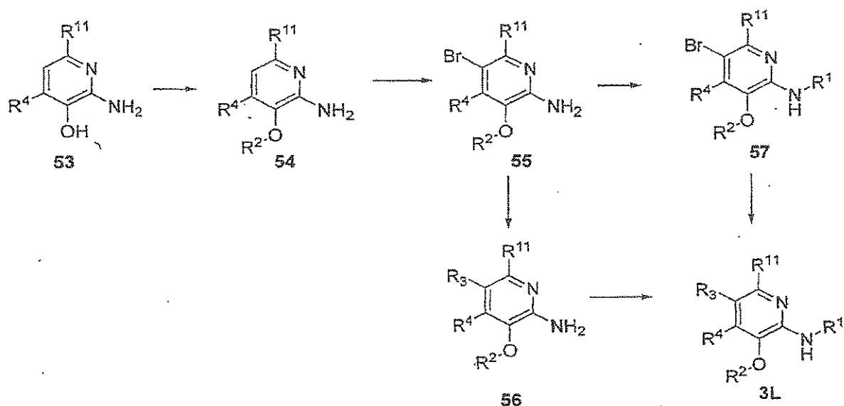
Scheme Q
