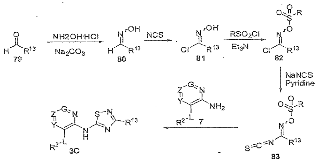
Scheme V
