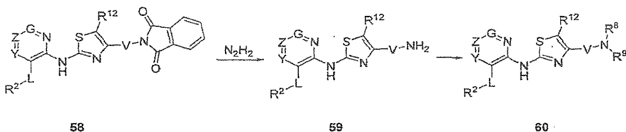
Scheme R
