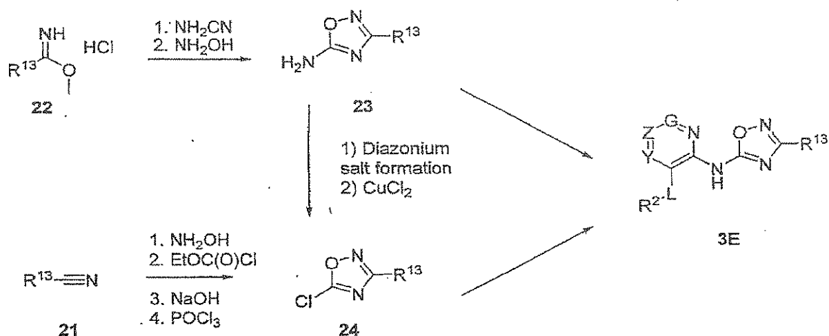
Scheme G
