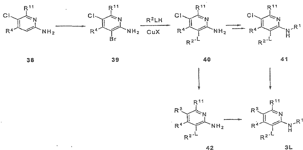
Scheme N
