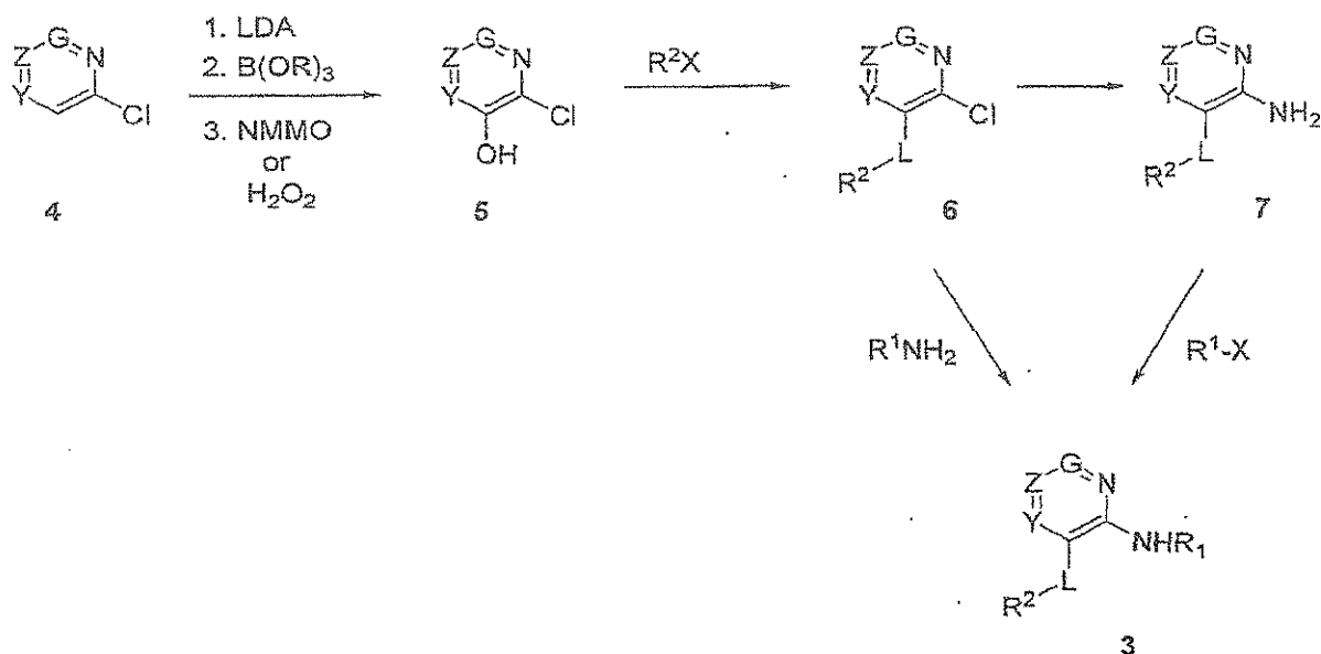
Scheme B
