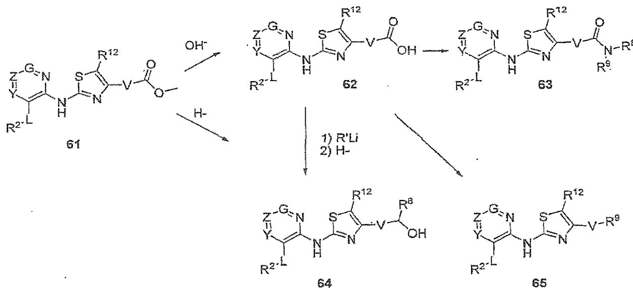
Scheme S
