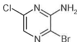
(a) 3-Bromo-6-chloro-2-pyrazinamine
