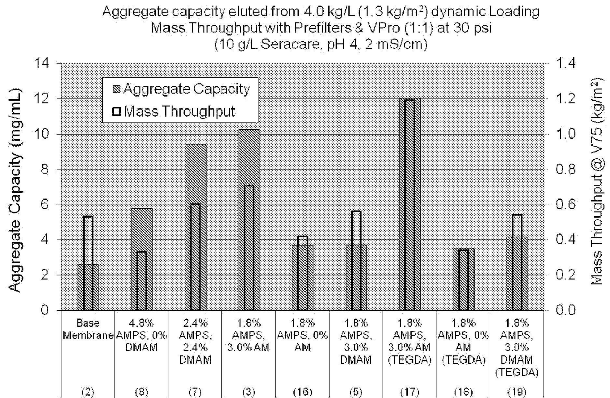
Figure 8. Aggregate binding capacities for IgG of various CEX surface-modified membranes and corresponding VPro throughput.
