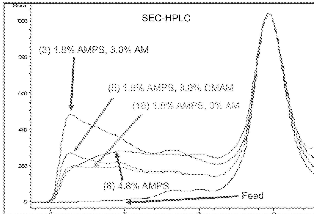
Figure 9. SEC chromatograms of elution IgG samples of various CEX surface-modified membranes.
