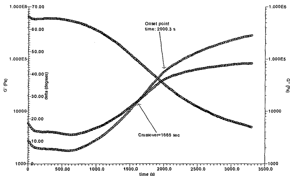
Graph 1. Parallel Plate Rheology of Blend 3, at 380 °C. See, J. Mercel et al. , "Thermal Analysis of Polymers: Fundamentals and Applications," p. 445, Wiley, ed. 1 (2009).
