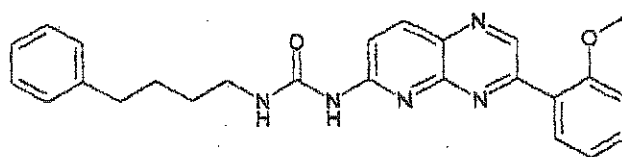
Compound 124: 1-[3-(2-Methoxy-phenyl)-pyrido[2,3-b]pyrazin-6-yl]-3-(4-phenyl-butyl)-urea
