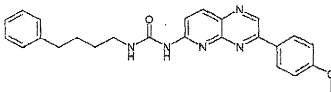
Compound 118: 1-[3-(4-Methoxy-phenyl)-pyrido[2,3-b]pyrazin-6-yl]-3-(4-phenyl-butyl)-urea
