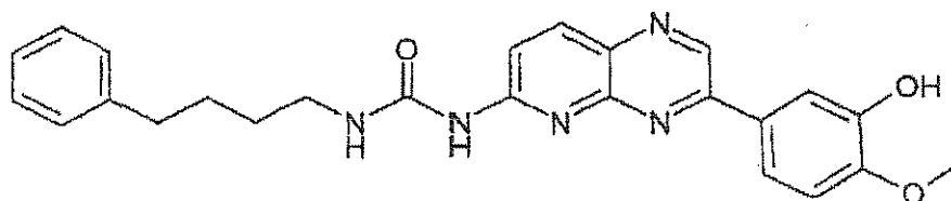
Compound 151: 1-[3-(3-Hydroxy-4-methoxy-phenyl)-pyrido[2,3-b]pyrazin-6-yl]-3-(4-phenyl-butyl)-urea
