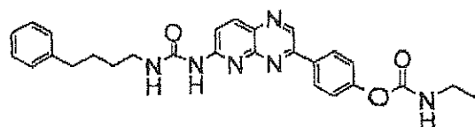
Compound 123: 1-[3-(4-Amino-3-methoxy-phenyl)-pyrido[2,3-b]pyrazin-6-yl]-3-(4-phenyl-butyl)-urea
