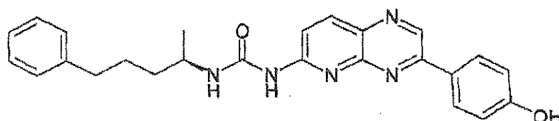
Compound 147: 1-[3-(4-Hydroxy-phenyl)-pyrido[2,3-b]pyrazin-6-yl]-3-((R)-1-methyl-4-phenyl-butyl)-urea
