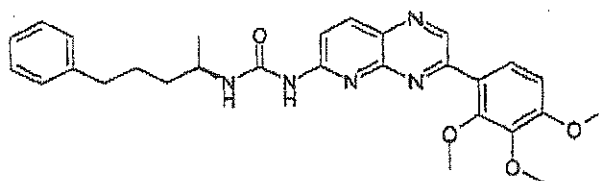
Compound 126: 1-(1-Methyl-4-phenyl-butyl)-3-[3-(1-propyl-1H-pyrazol-4-yl)-pyrido[2,3-b]pyrazin-6-yl]-urea
