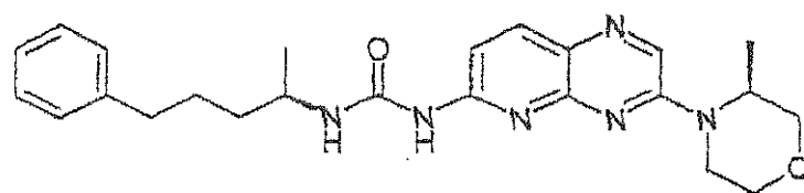
Compound 187: 1-[3-((S)-3-Methyl-morpholin-4-yl)-pyrido[2,3-b]pyrazin-6-yl]-3-((R)-1-methyl-4-phenyl-butyl)-urea
