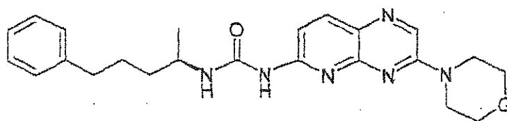
Compound 172: 1-(4-Phenyl-butyl)-3-(3-pyrrolidin-1-yl-pyrido[2,3-b]pyrazin-6-yl)-urea
