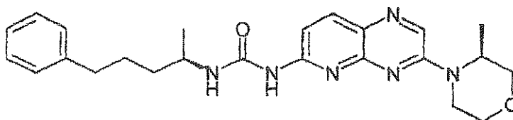
15 Compound 187: 1-[3-((S)-3-Methyl-morpholin-4-yl)-pyrido[2,3-b]pyrazin-6-yl]-3-((R)-1-methyl-4-phenyl-butyl)-urea
