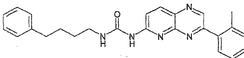
Compound 120: 1-(4-Phenyl-butyl)-3-(3-o-tolyl-pyrido[2,3-b]pyrazin-6-yl)-urea
