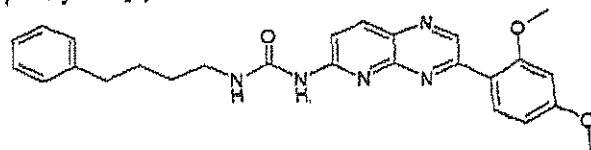
Compound 101: 1-[3-(2,4-Dimethoxy-phenyl)-pyrido[2,3-b]pyrazin-6-yl]-3-(4-phenyl-butyl)-urea
