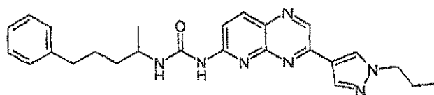
Compound 126: 1-(1-Methyl-4-phenyl-butyl)-3-[3-(1-propyl-1H-pyrazol-4-yl)-pyrido[2,3-b]pyrazin-6-yl]-urea
