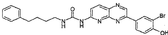
Compound 110: 1-(4-Phenyl-butyl)-3-(3-pyridin-3-yl-pyrido[2,3-b]pyrazin-6-yl)-urea
