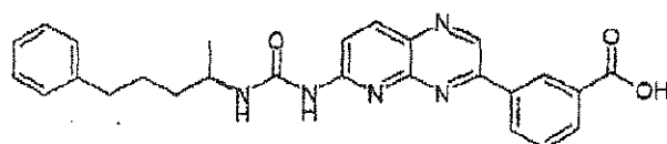
Compound 196: 3-[6-[3-((R)-1-Methyl-4-phenyl-butyl)-ureido]-pyrido[2,3-b]pyrazin-3-yl]-benzoic acid
