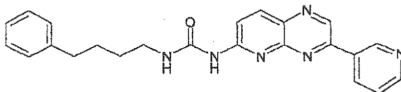
Compound 110: 1-(4-Phenyl-butyl)-3-(3-pyridin-3-yl-pyrido[2,3-b]pyrazin-6-yl)-urea
