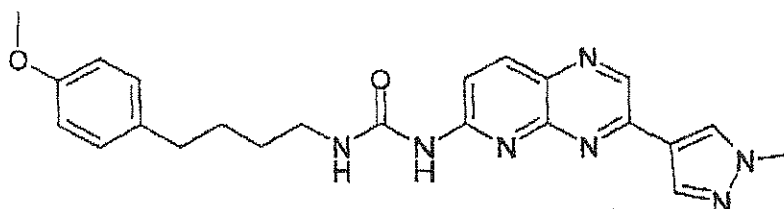
Compound 118: 1-[3-(4-Methoxy-phenyl)-pyrido[2,3-b]pyrazin-6-yl]-3-(4-phenyl-butyl)-urea
