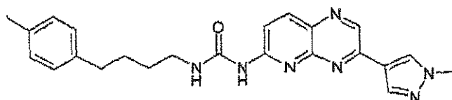
Compound 98: 1-[3-(3,4-Dimethoxy-phenyl)-pyrido[2,3-b]pyrazin-6-yl]-3-((R)-1-methyl-4-phenyl-butyl)-urea
