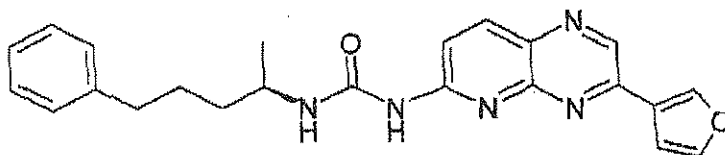
Compound 150: 1-((R)-1-Methyl-4-phenyl-butyl)-3-(3-pyridin-3-yl-pyrido[2,3-b]pyrazin-6-yl)-urea
