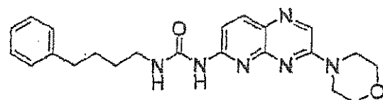
Compound 187: 1-[3-((S)-3-Methyl-morpholin-4-yl)-pyrido[2,3-b]pyrazin-6-yl]-3-((R)-1-methyl-4-phenyl-butyl)-urea
