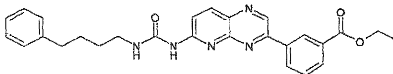
Compound 122: Ethyl-carbamic acid 4-{6-[3-(4-phenyl-butyl)-ureido]-pyrido[2,3-b]pyrazin-3-yl}-phenyl ester
