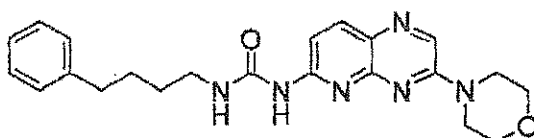
15 Compound 187: 1-[3-((S)-3-Methyl-morpholin-4-yl)-pyrido[2,3-b]pyrazin-6-yl]-3-((R)-1-methyl-4-phenyl-butyl)-urea
