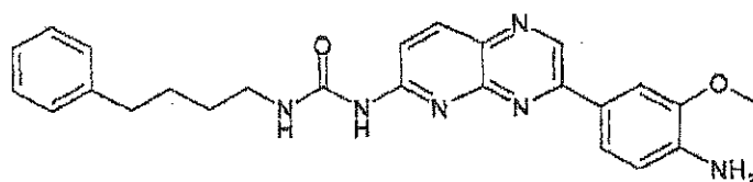
Compound 123: 1-[3-(4-Amino-3-methoxy-phenyl)-pyrido[2,3-b]pyrazin-6-yl]-3-(4-phenyl-butyl)-urea
