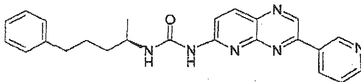
Compound 150: 1-((R)-1-Methyl-4-phenyl-butyl)-3-(3-pyridin-3-yl-pyrido[2,3-b]pyrazin-6-yl)-urea
