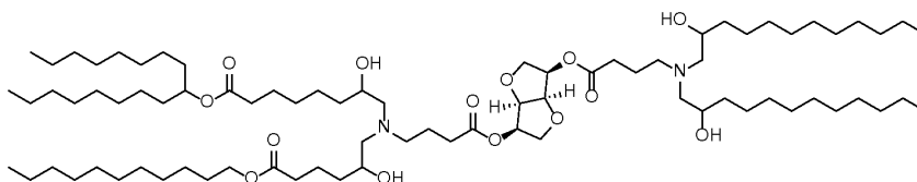
Compound 9
