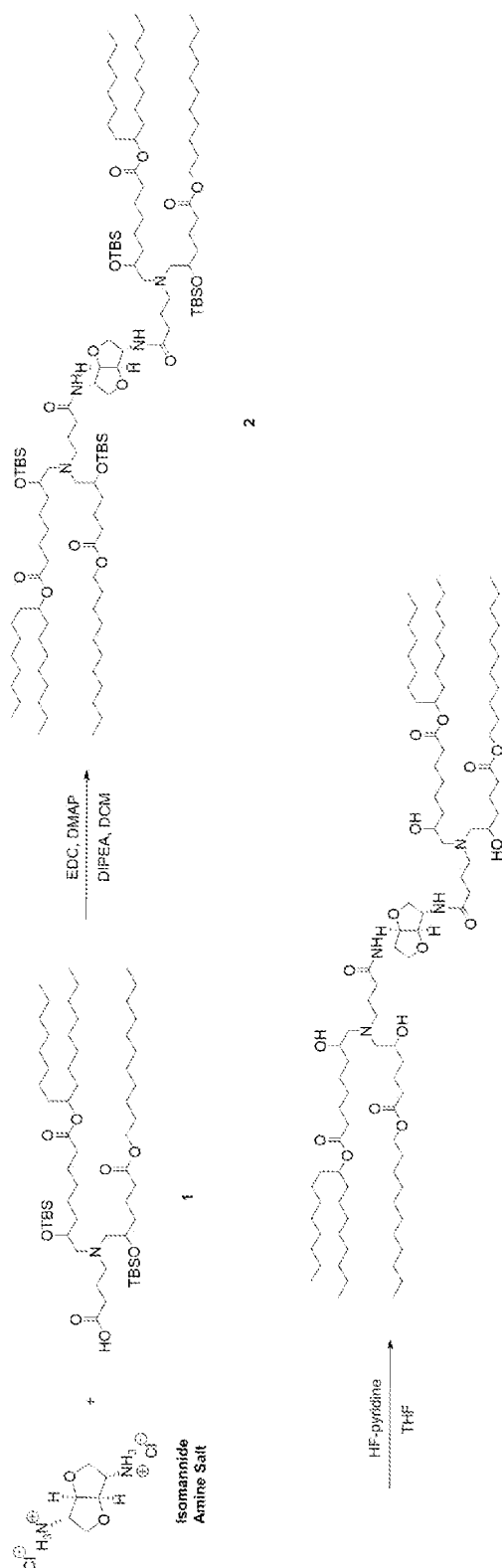
Compound 73
