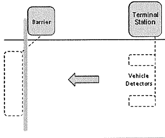
Fig. 2 Example of equipment at a Typical car park Lane control point
