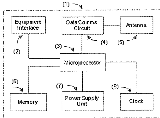
Fig. 1 The invented device
