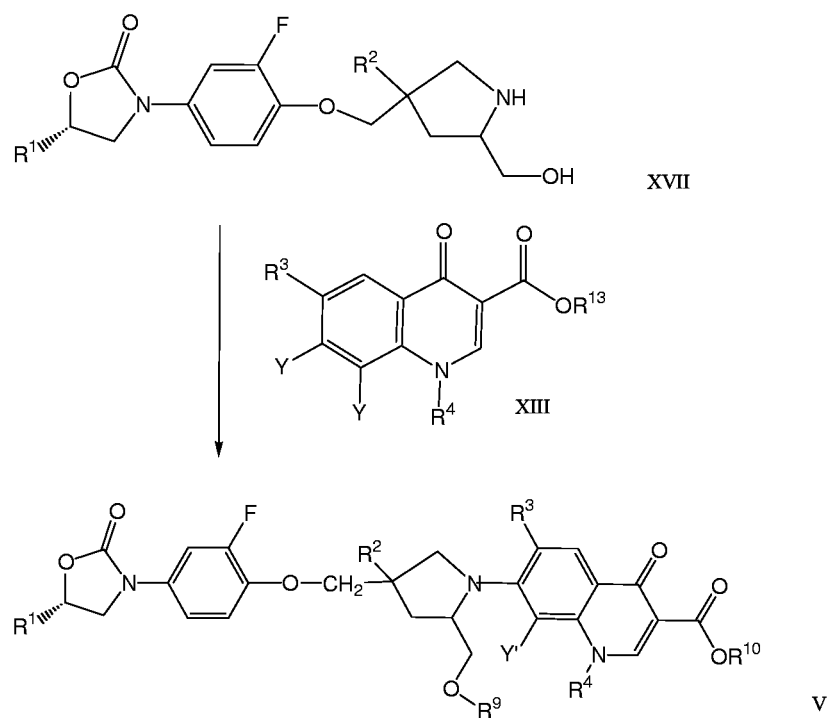
Scheme 4
