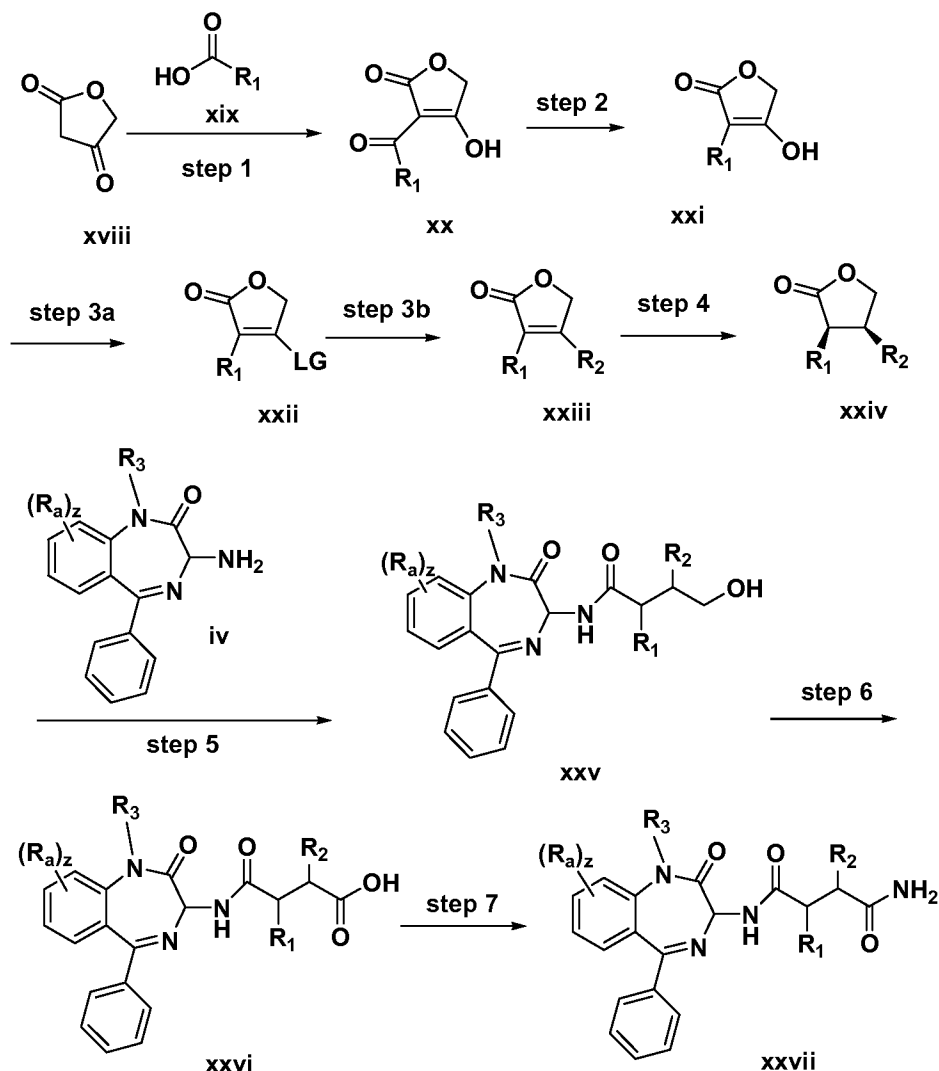
Scheme 4
