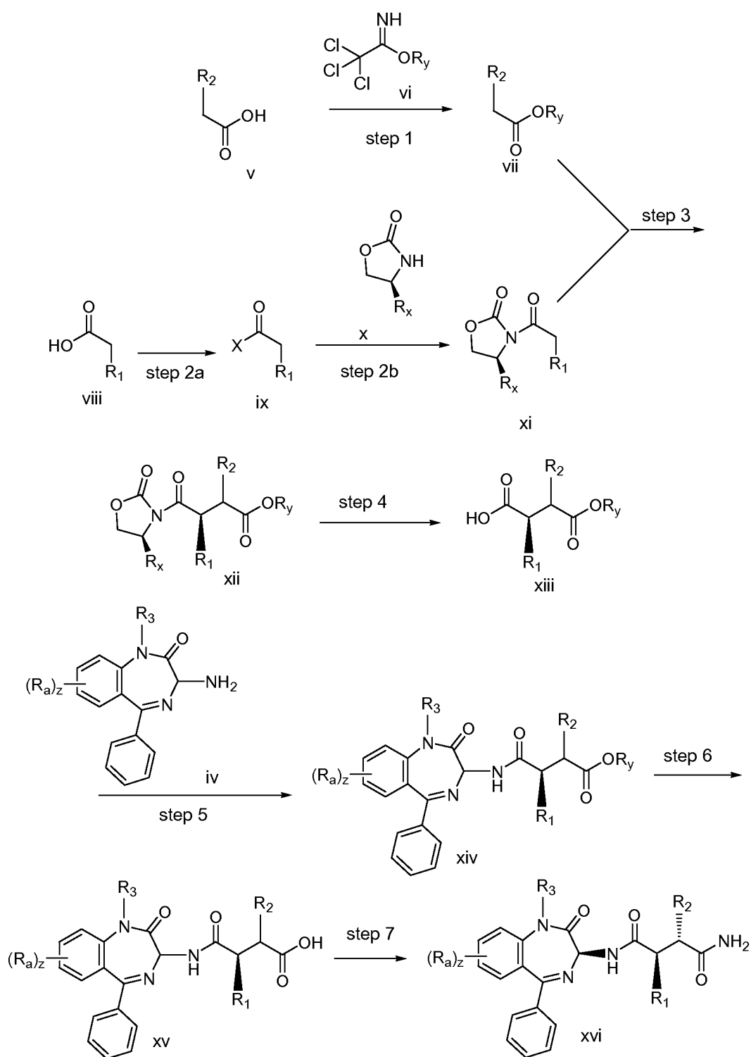
Scheme 2
