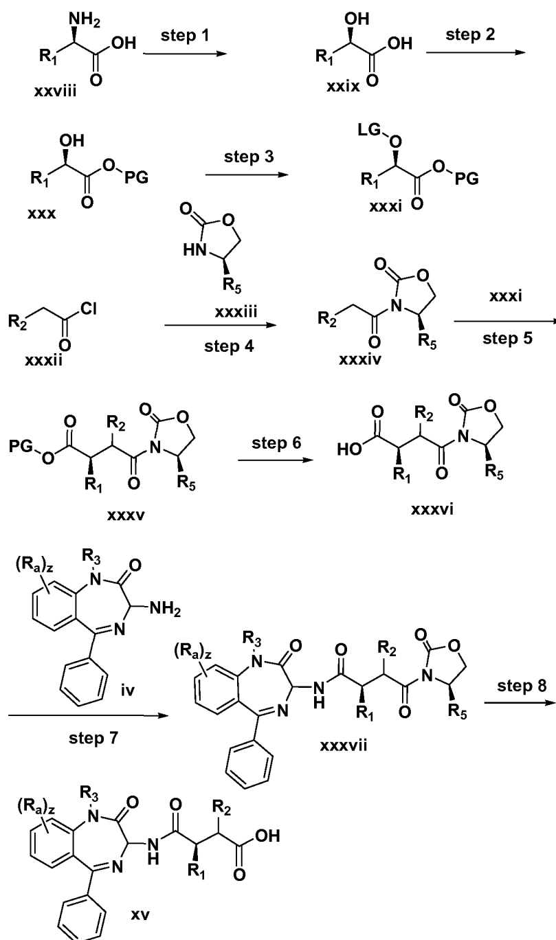
Scheme 5
