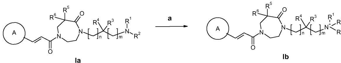
Scheme 5
