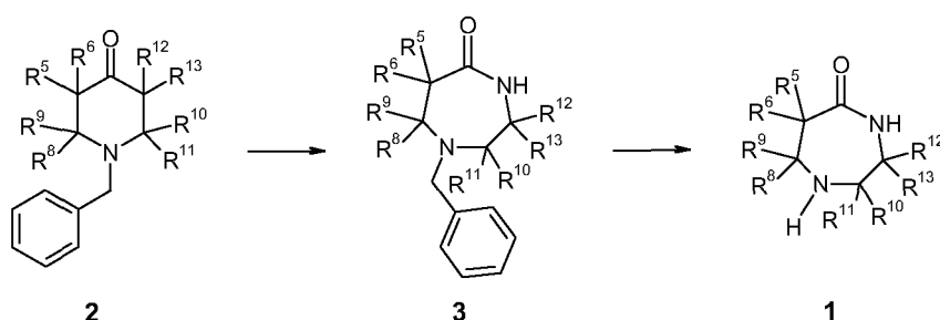
Scheme 7
