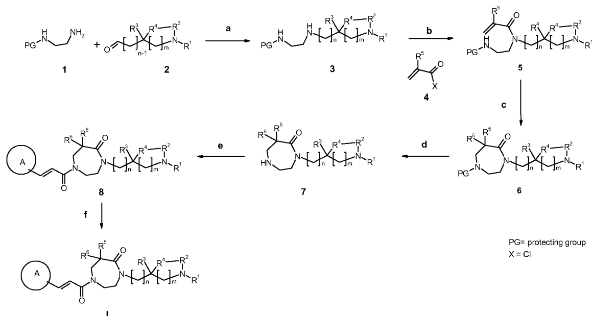
Scheme 4
