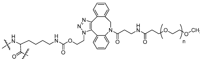
Formula (X)
