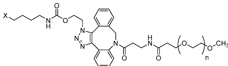
Formula (VI)
