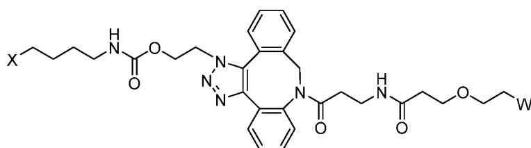
XCCCCNC(=O)OCCN1N=NC2=C1C3=CC=CC=C3N(C2)C(=O)CCNC(=O)CCOCCW
