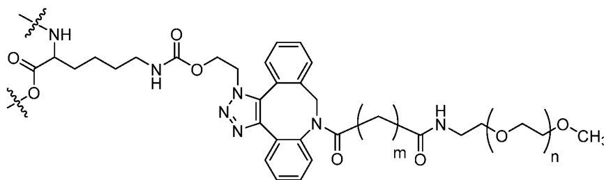
Formula (XVI)
