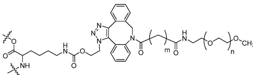
Formula (XVII)
