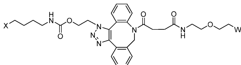
Formula (V);
