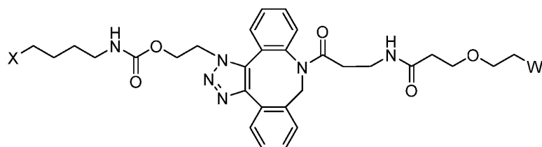
Formula (III);
