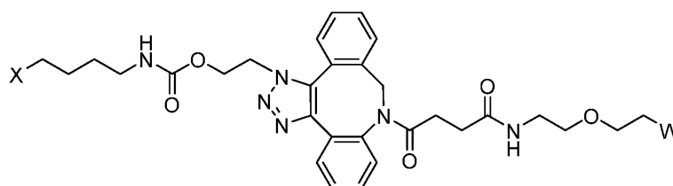
Formula (IV);
