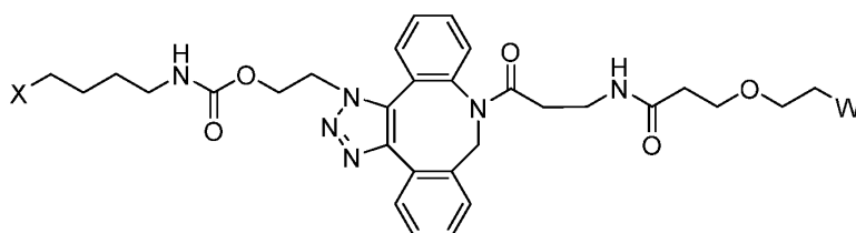
Formula (III);
