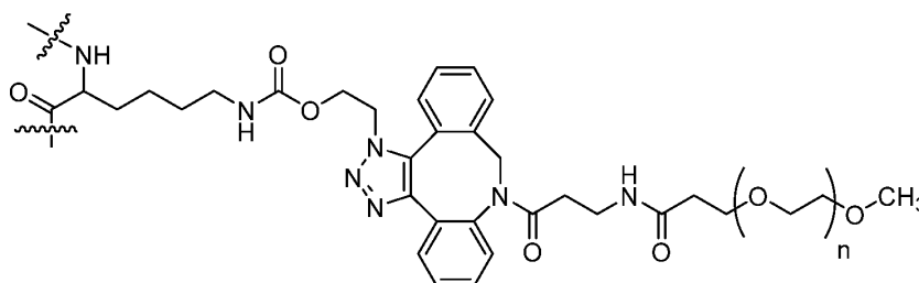
Formula (XI)
