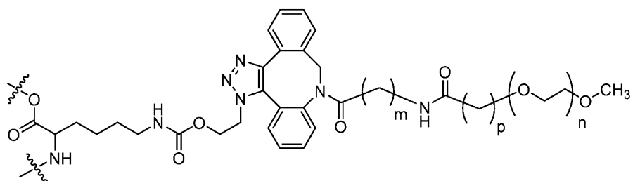
Formula (XV)
