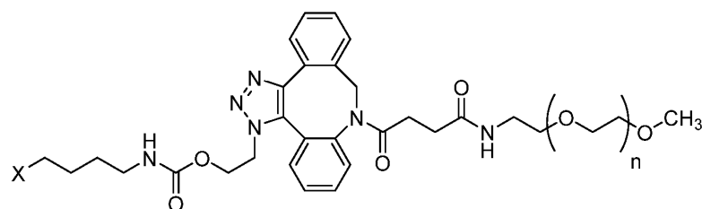
Formula (IX)
