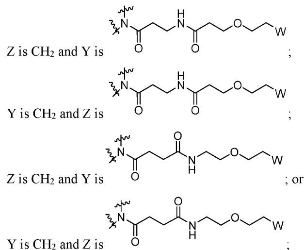
Formula (I);
