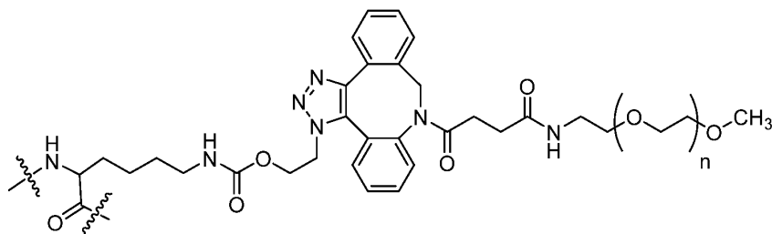
Formula (XIII)
