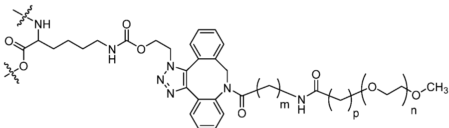
Formula (XIV)
