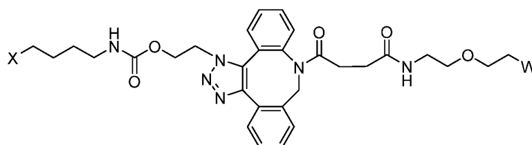
Formula (V);
