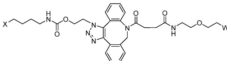
Formula (V);
