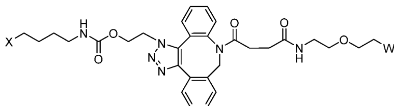
Formula (V);
