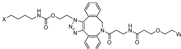
Formula (II);
