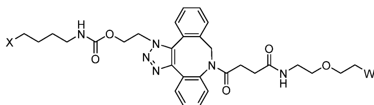
Formula (IV);
