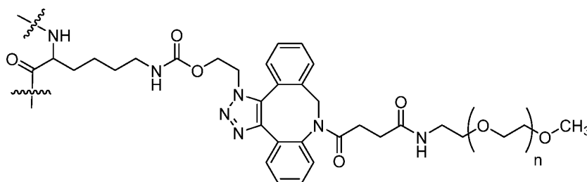
Formula (XII)
