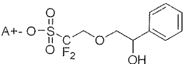
[Chemical Formula 3-5]
