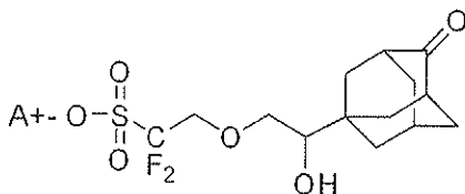
[Chemical Formula 3-8]
