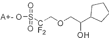
[Chemical Formula 3-11]
