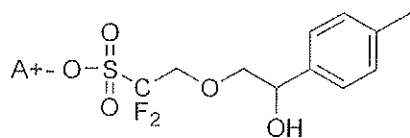
[Chemical Formula 3-7]
