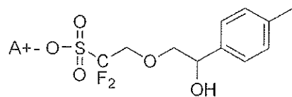
[Chemical Formula 3-7]
