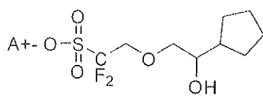
[Chemical Formula 3-11]
