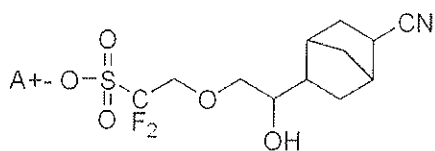
[Chemical Formula 3-10]
