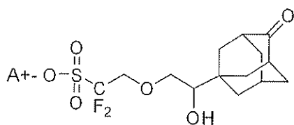
[Chemical Formula 3-8]
