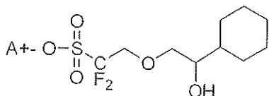
[Chemical Formula 3-3]
