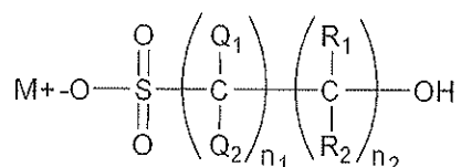
[Chemical Formula 7]
