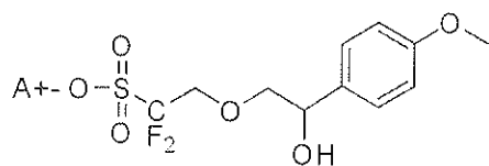
[Chemical Formula 3-12]
