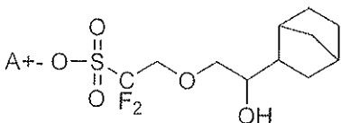
[Chemical Formula 3-4]
