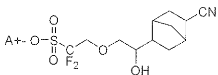
[Chemical Formula 3-10]
