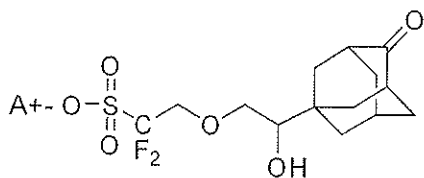
[Chemical Formula 3-8]
