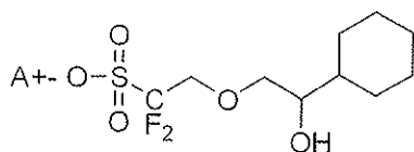
[Chemical Formula 3-3]
