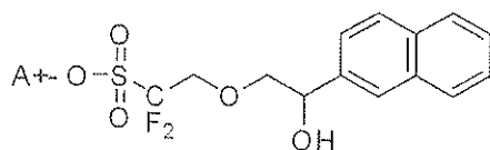
[Chemical Formula 3-6]
