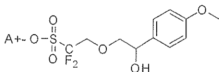
[Chemical Formula 3-12]
