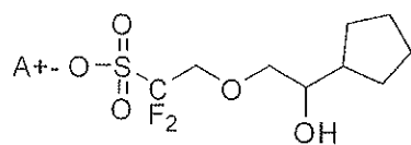
[Chemical Formula 3-11]
