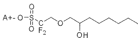
[Chemical Formula 3-12]
