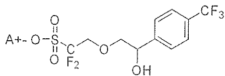
[Chemical Formula 3-9]
