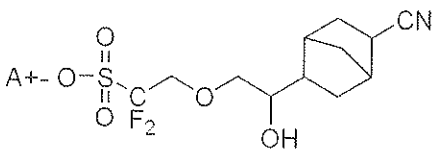
[Chemical Formula 3-10]
