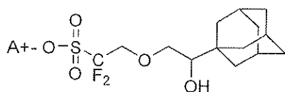
[Chemical Formula 3-2]
