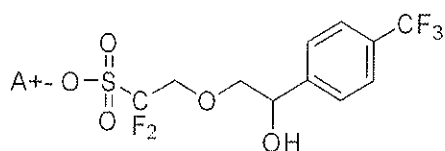
[Chemical Formula 3-9]
