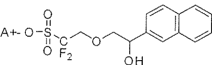
[Chemical Formula 3-5]
