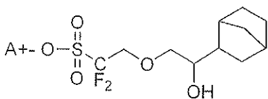
[Chemical Formula 3-4]
