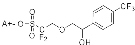
[Chemical Formula 3-9]
