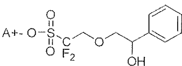
[Chemical Formula 3-5]
