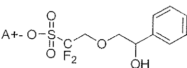
[Chemical Formula 3-5]
