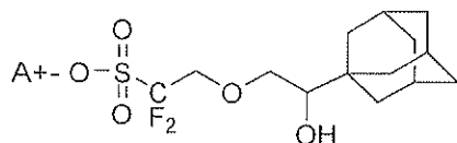
[Chemical Formula 3-2]
