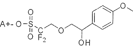
[Chemical Formula 3-12]
