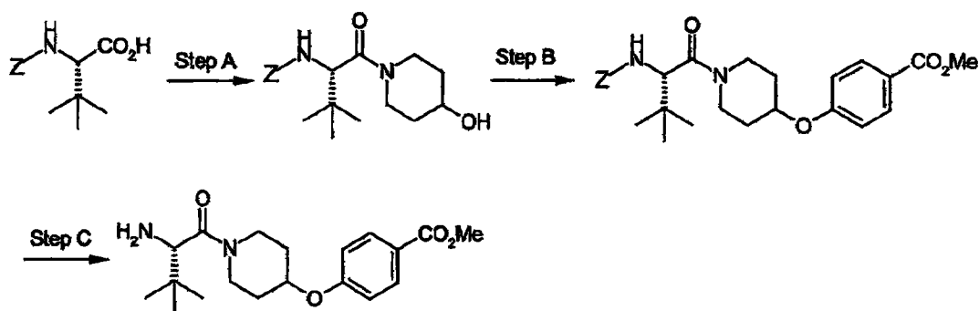
Scheme 7
