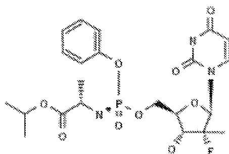
PSI-7977
