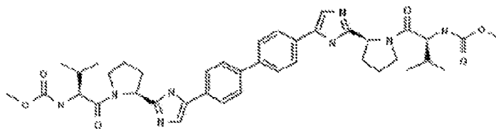
Daclatasvir dihydrochloride
