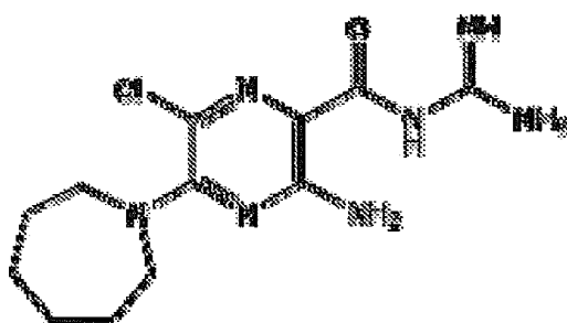
BIT-225
