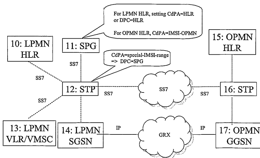
Signal Packet Gateway Network Architecture
