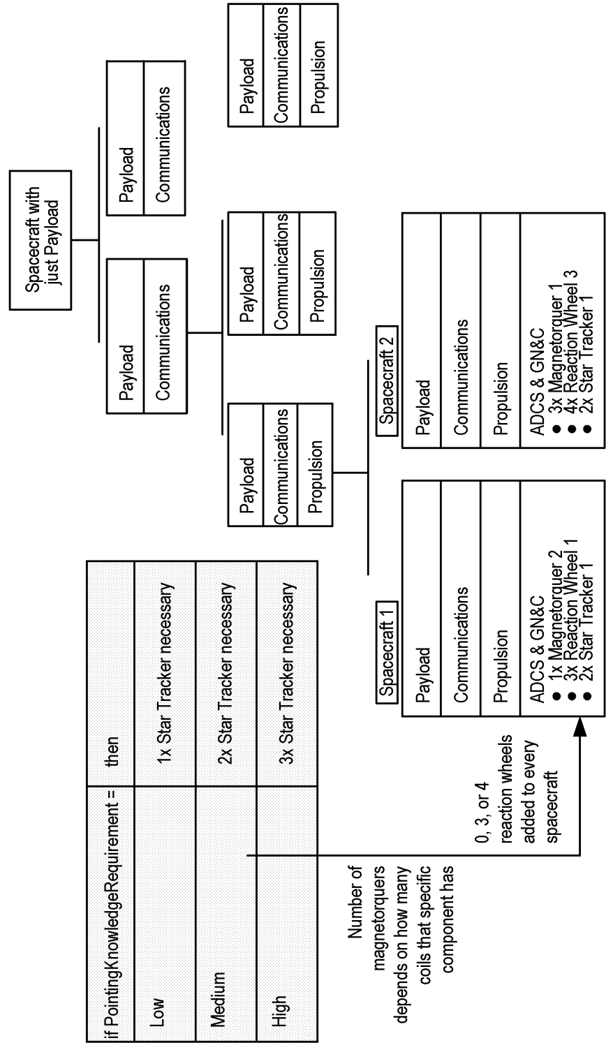
ADCS and GN&C Subsystem Selection
