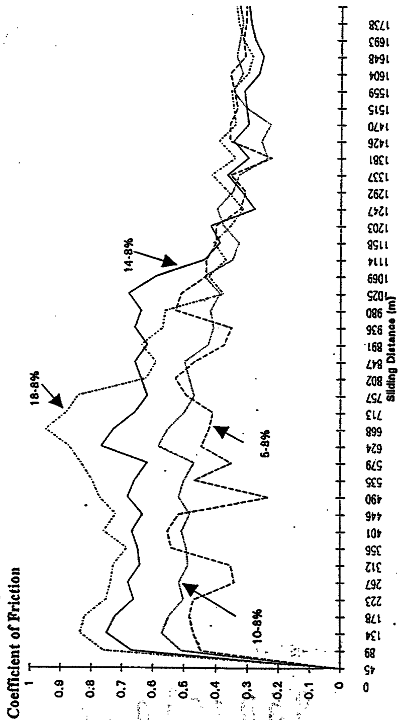
Figure 2(b) : Coefficient of Friction of the various 8% graphite composites
